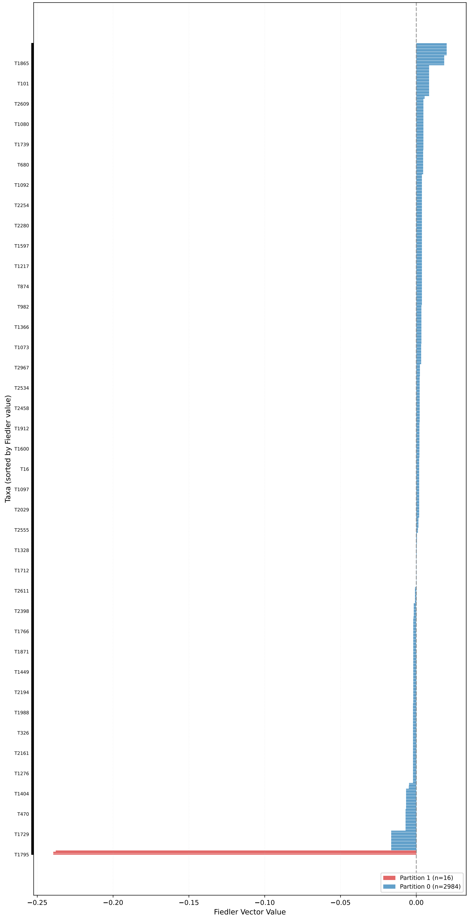
Partition for kingman_mean_pop_100 (n=3000, L=10000, \mu=0.20 ) - Fiedler Vector \sigma_2=0.0001 , Gap=0.0001, Coherence=0.0119
