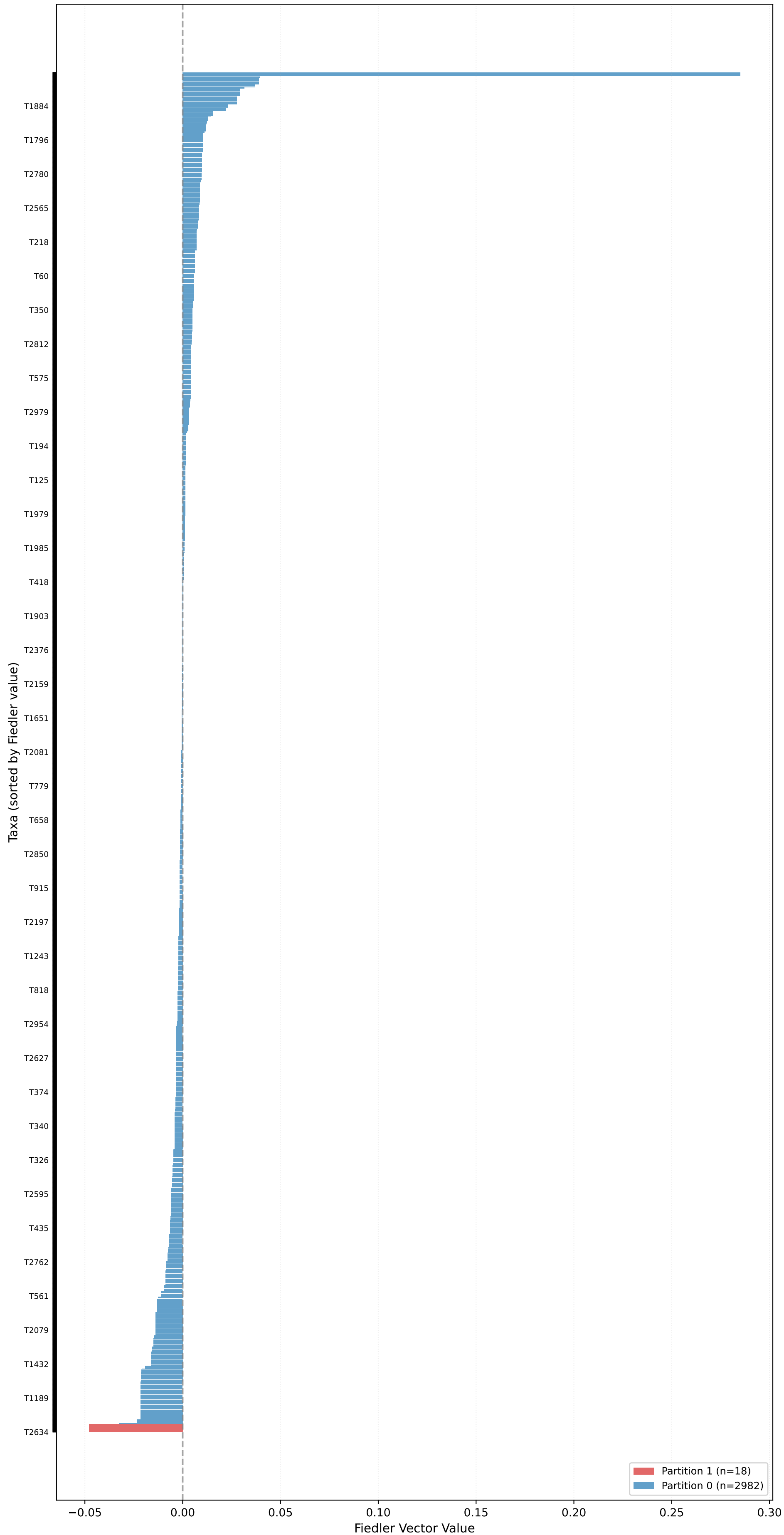
Partition for kingman_mean_pop_1000 (n=3000, L=10000, \mu=0.10 ) - Fiedler Vector \sigma_2=0.0001 , Gap=0.0000, Coherence=0.0791
