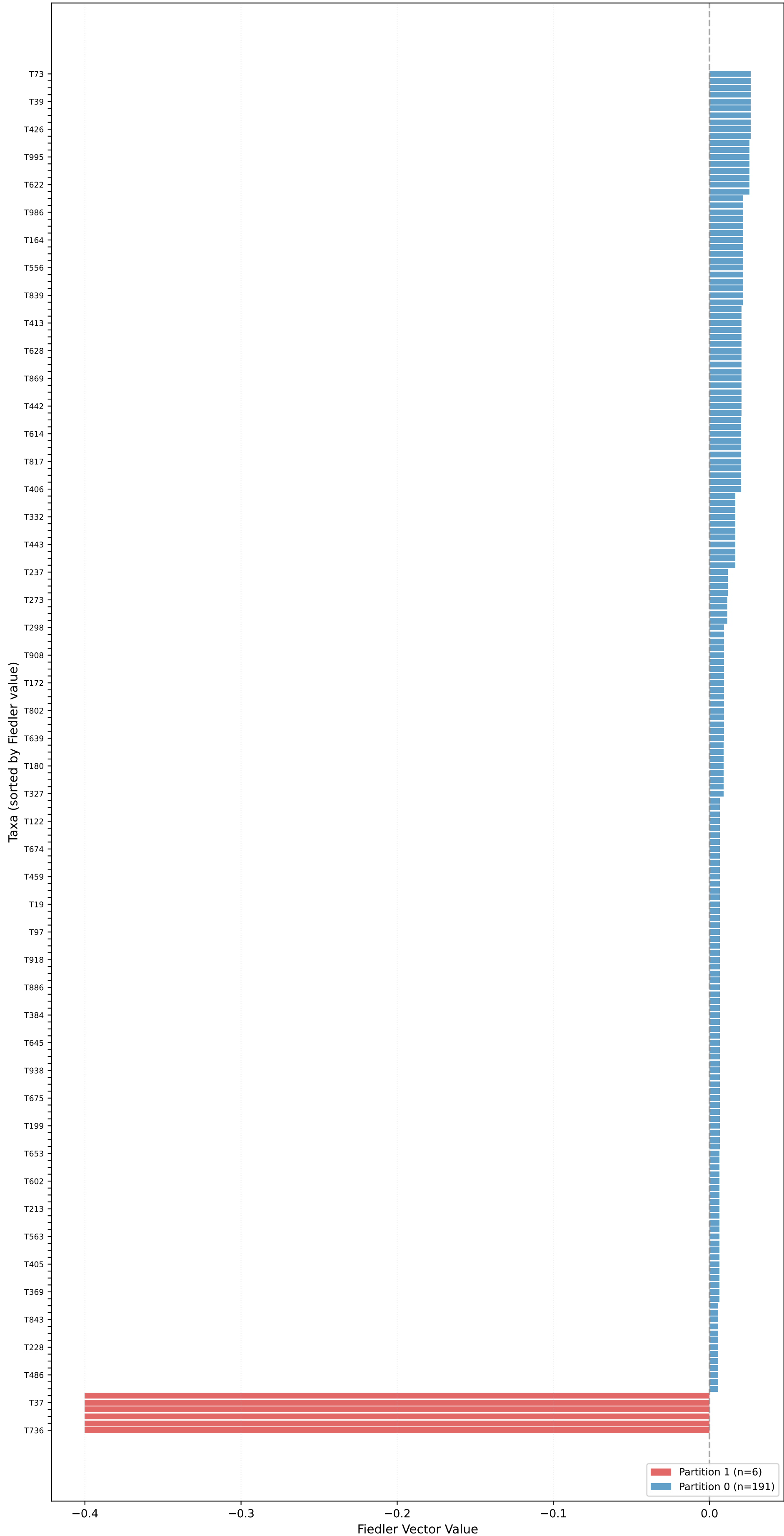
Partition for extinction_heavy (n=1000, L=10000, \mu=0.10 ) - Fiedler Vector \sigma_2=0.0000 , Gap=0.0000, Coherence=0.1560
