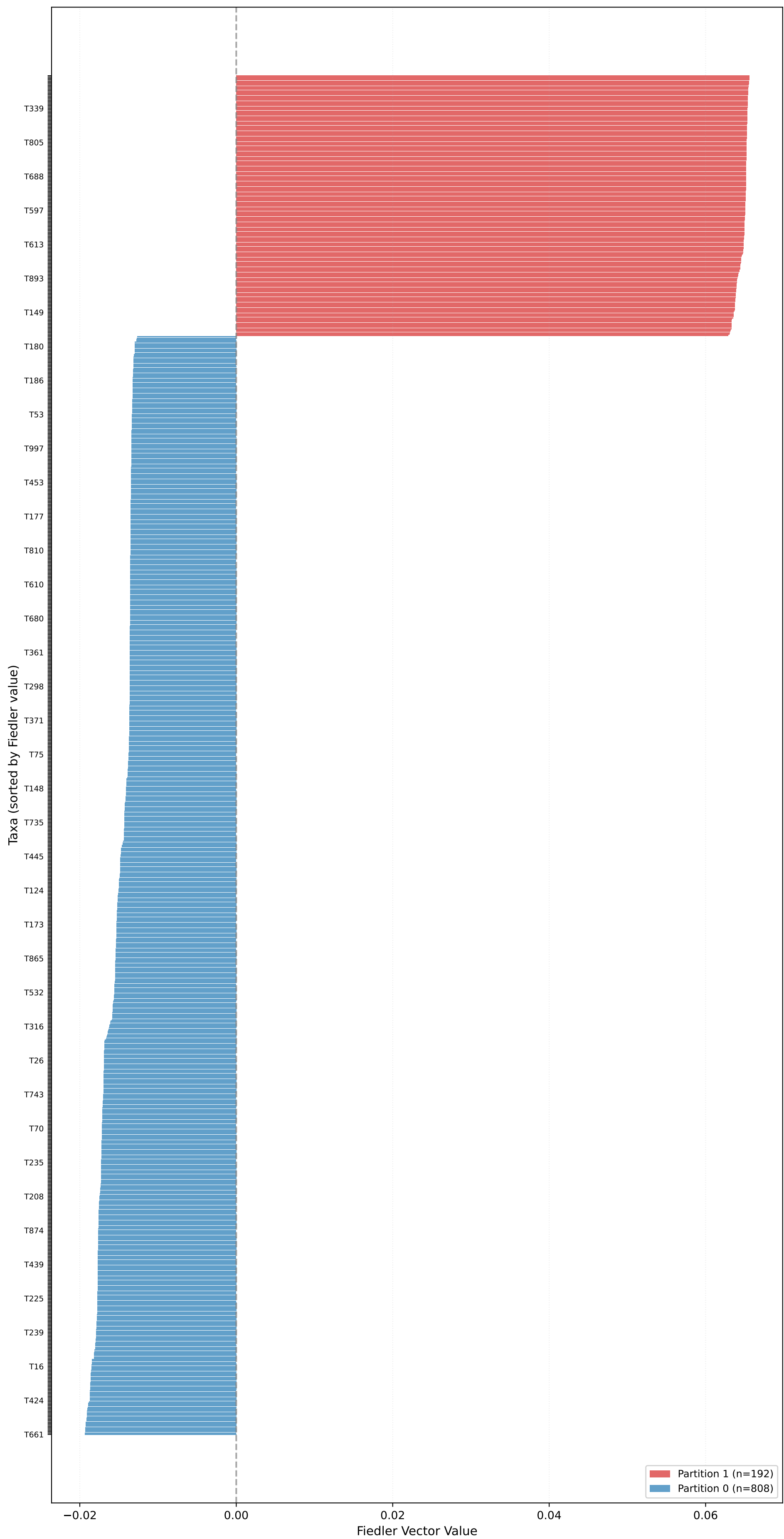
Partition for yule_pure_birth (n=1000, L=10000, \mu=0.10 ) - Fiedler Vector \sigma_2=0.0031 , Gap=0.0380, Coherence=0.0503
