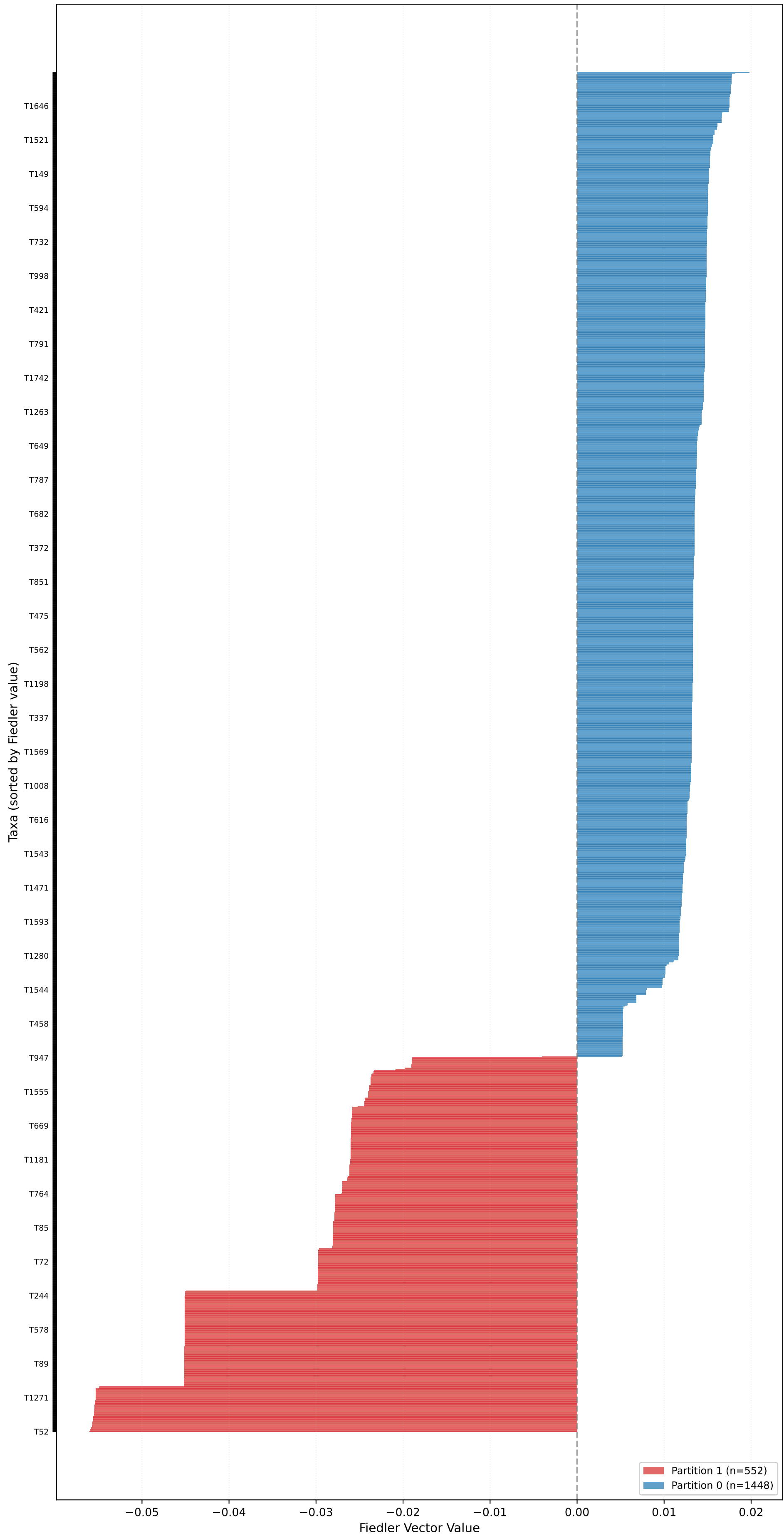
Partition for yule_pure_birth (n=2000, L=10000, \mu=0.20 ) - Fiedler Vector \sigma_2=0.0001 , Gap=0.0001, Coherence=0.1448
