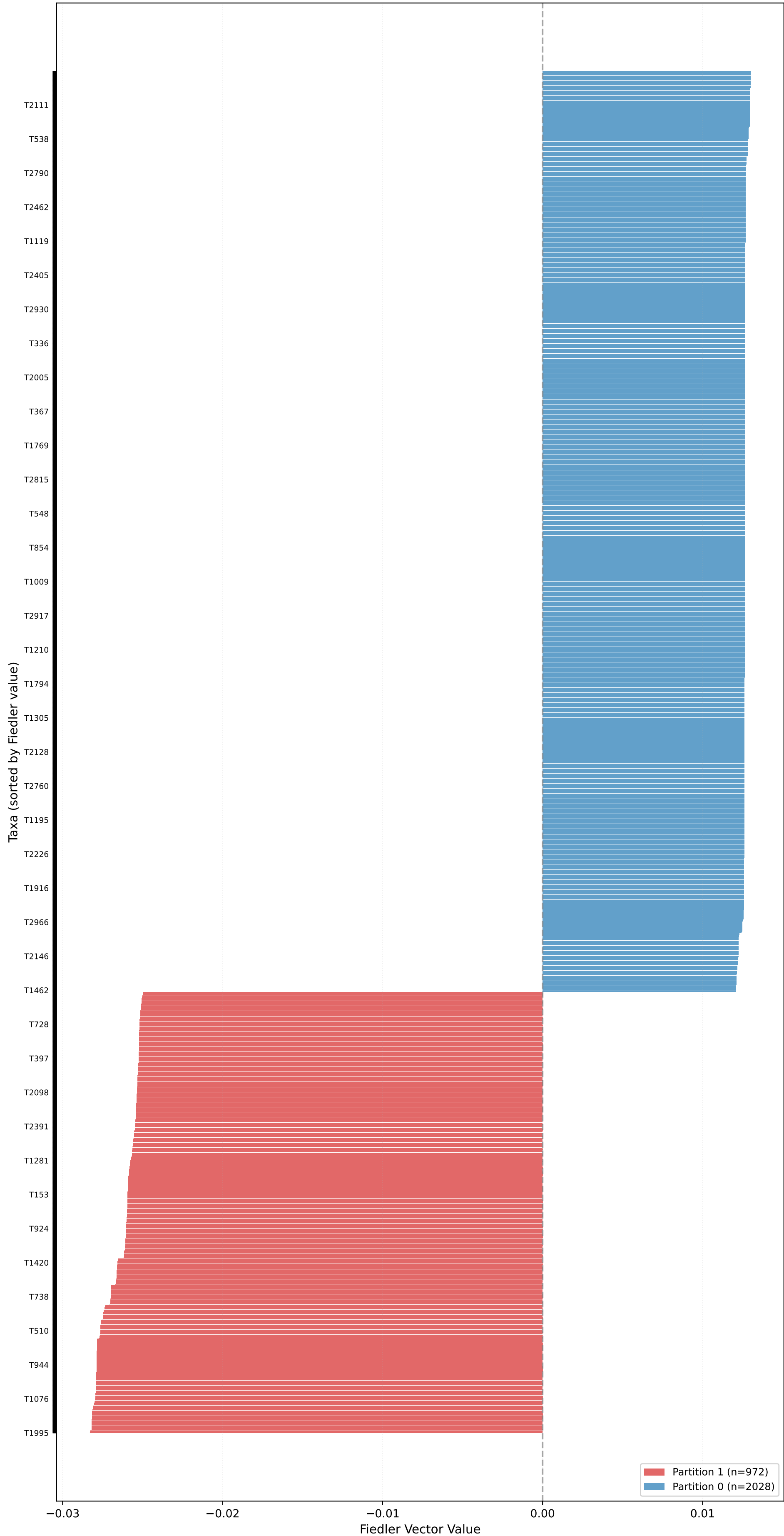
Partition for yule_pure_birth (n=3000, L=10000, \mu=0.10 ) - Fiedler Vector \sigma_2=0.0007 , Gap=0.0020, Coherence=0.0885
