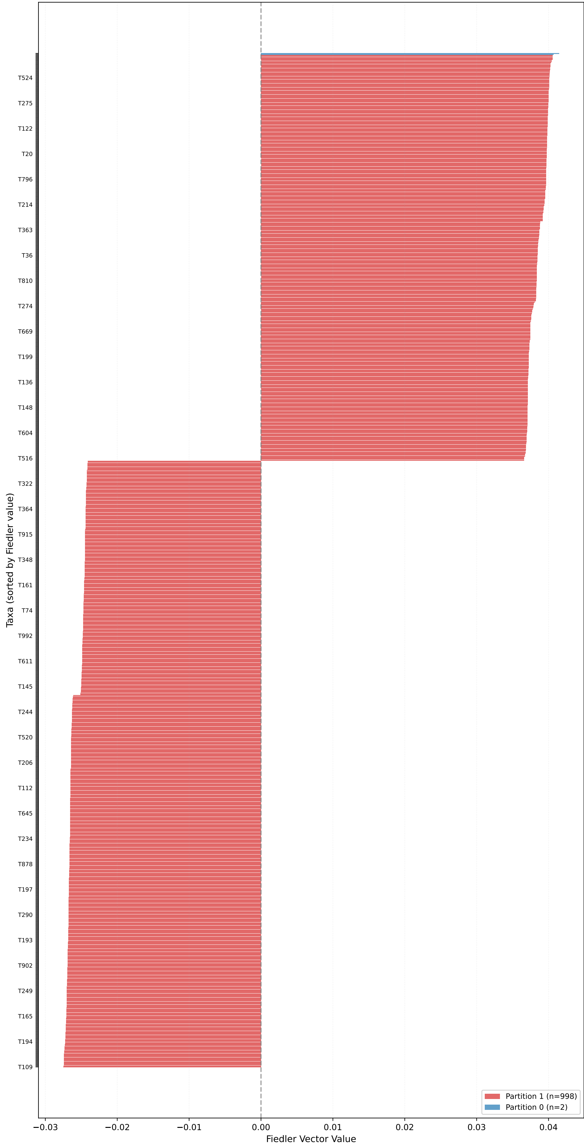
Partition for kingman_mean_pop_0.1 (n=1000, L=10000, \mu=0.20 ) - Fiedler Vector \sigma_2=0.0842 , Gap=74.7033, Coherence=0.0017
