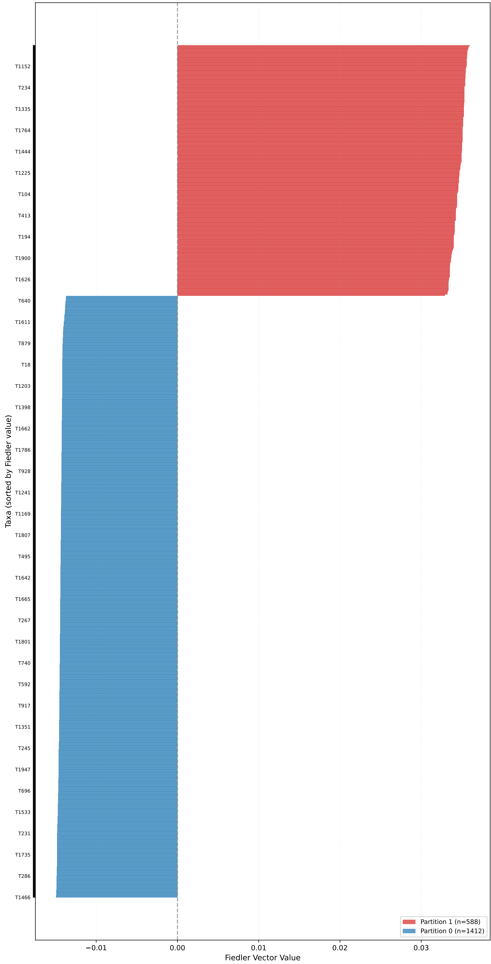
Partition for kingman_mean_pop_0.1 (n=2000, L=10000, \mu=0.20 ) - Fiedler Vector \sigma_2=0.2330 , Gap=131.7655, Coherence=0.0013
