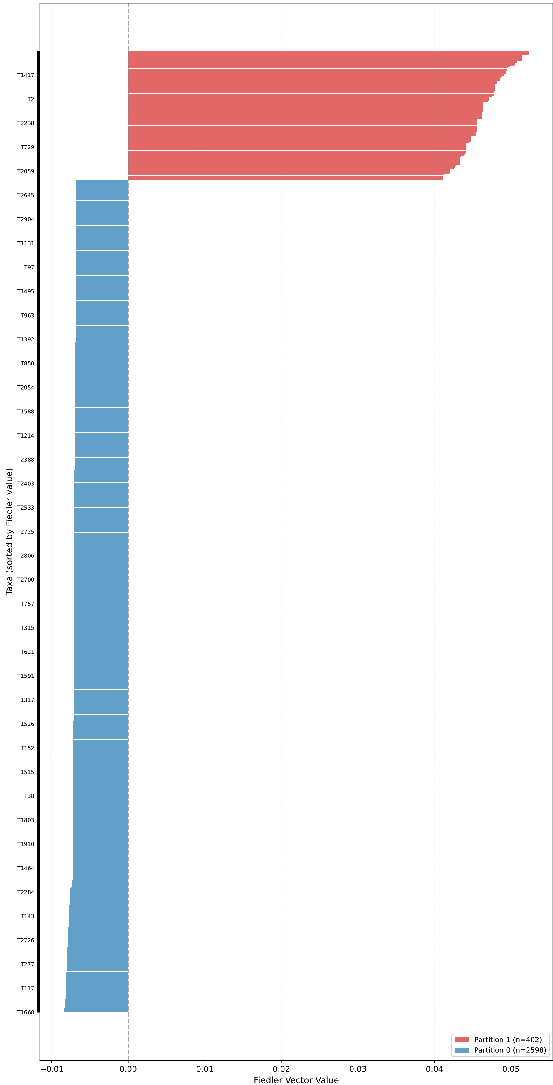
Partition for unrooted_pure_kingman_tree_pop_size_0.1 (n=3000, L=10000, \mu=0.20 ) - Fiedler Vector \sigma_2=0.1164 , Gap=56.0173, Coherence=0.0016
