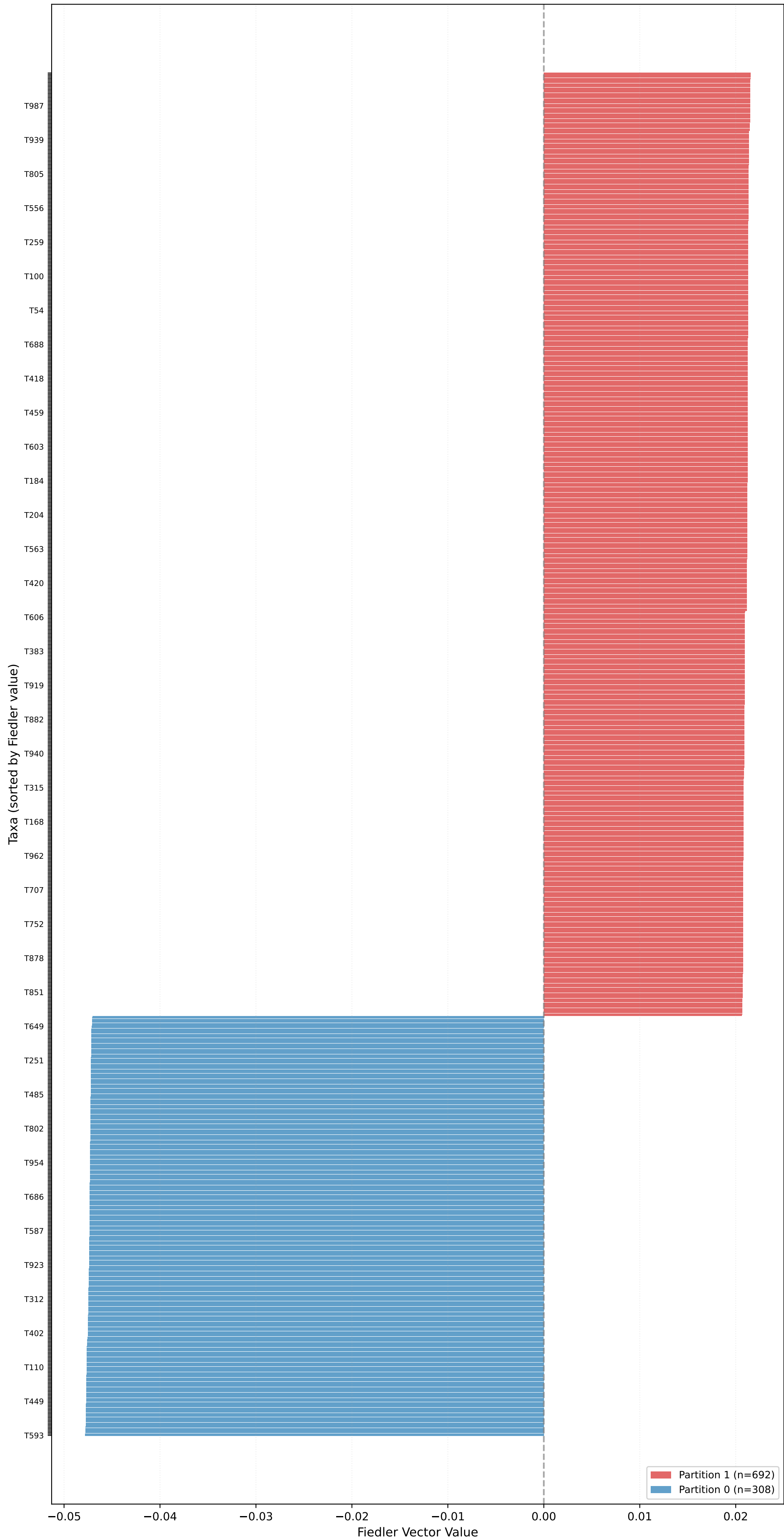
Partition for unrooted_pure_kingman_tree_pop_size_1.0 (n=1000, L=10000, \mu=0.10 ) - Fiedler Vector \sigma_2=0.1147 , Gap=128.5839, Coherence=0.0031
