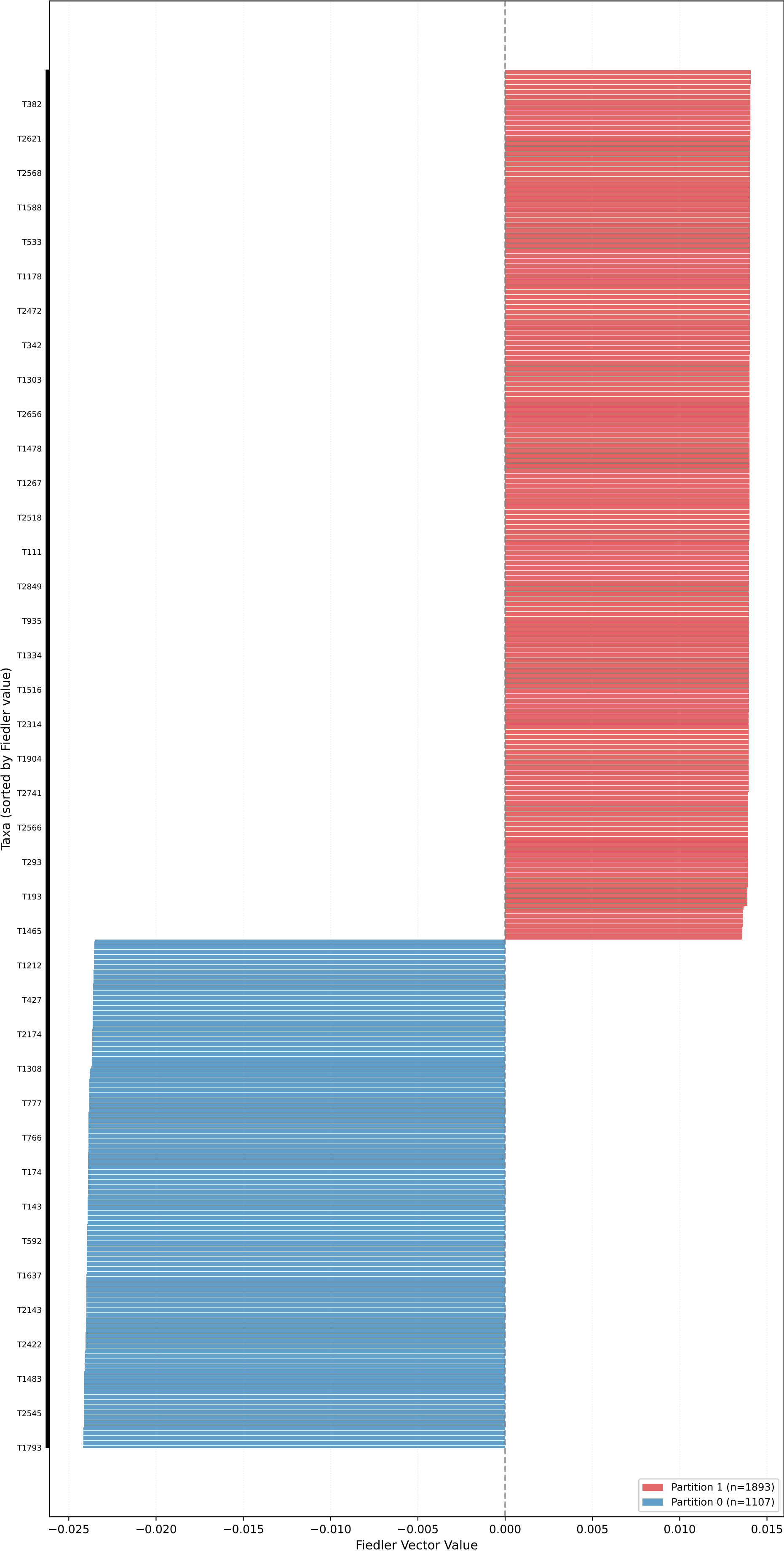
Partition for unrooted_pure_kingman_tree_pop_size_1.0 (n=3000, L=10000, \mu=0.20 ) - Fiedler Vector \sigma_2=0.5071 , Gap=170.2894, Coherence=0.0010
