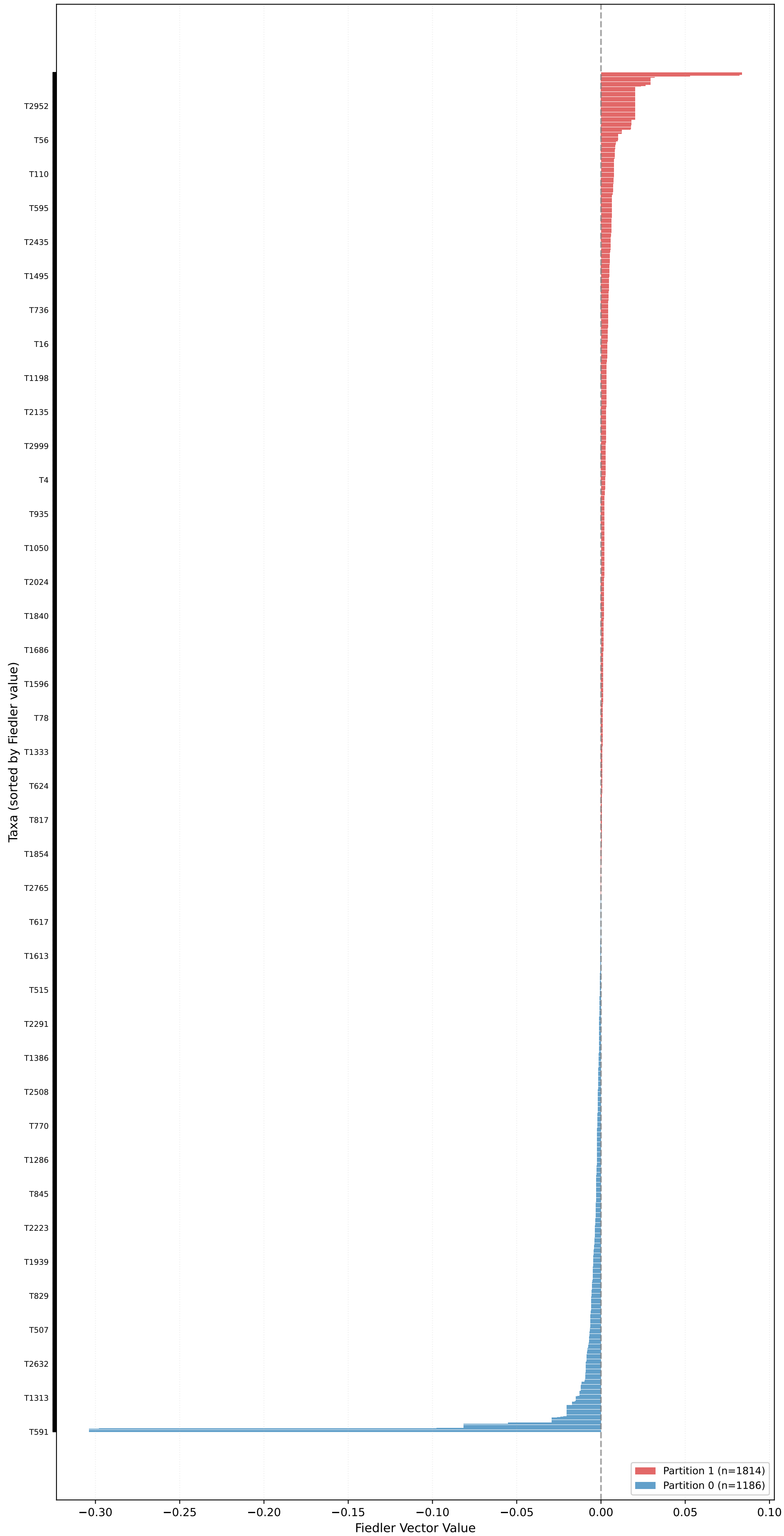
Partition for unrooted_pure_kingman_tree_pop_size_1000 (n=3000, L=10000, \mu=0.20 ) - Fiedler Vector \sigma_2=0.0013 , Gap=0.0000, Coherence=0.1490
