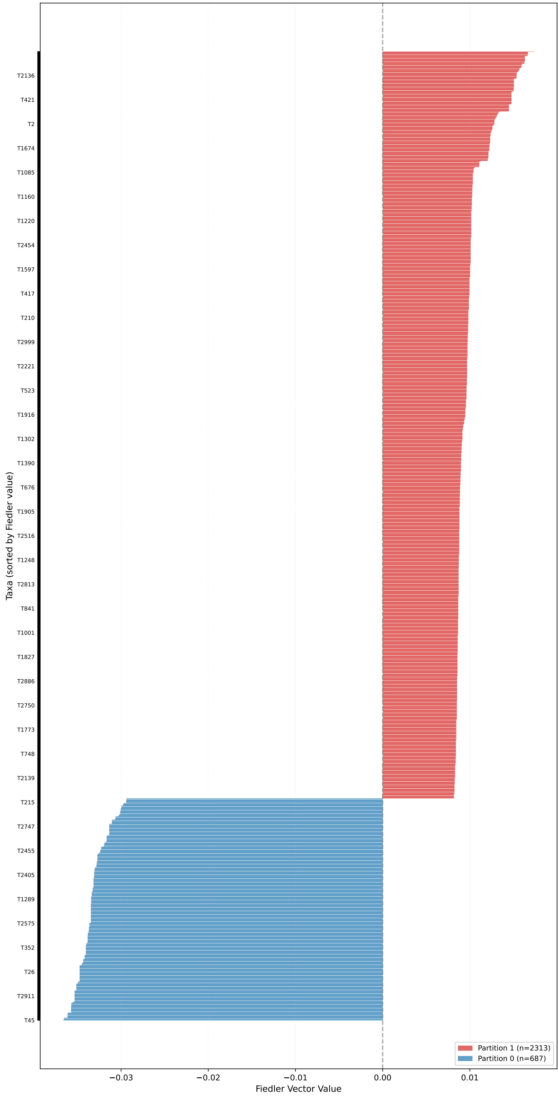
Partition for unrooted_pure_kingman_tree_pop_size_0.1 (n=3000, L=10000, \mu=0.20 ) - Fiedler Vector \sigma_2=0.2240 , Gap=23.8842, Coherence=0.0011
