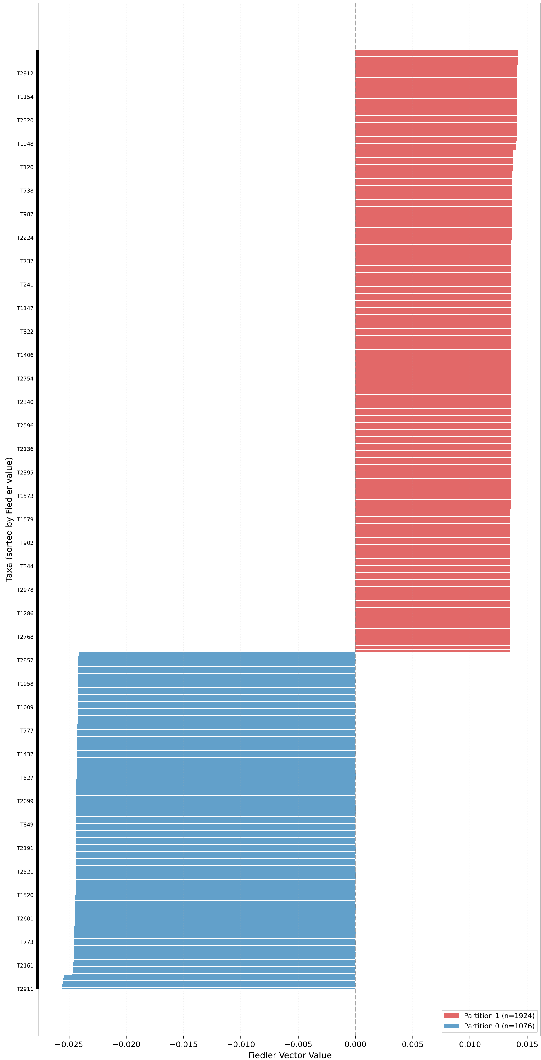
Partition for unrooted_pure_kingman_tree_pop_size_1.0 (n=3000, L=10000, \mu=0.10 ) - Fiedler Vector \sigma_2=0.5026 , Gap=456.3901, Coherence=0.0007
