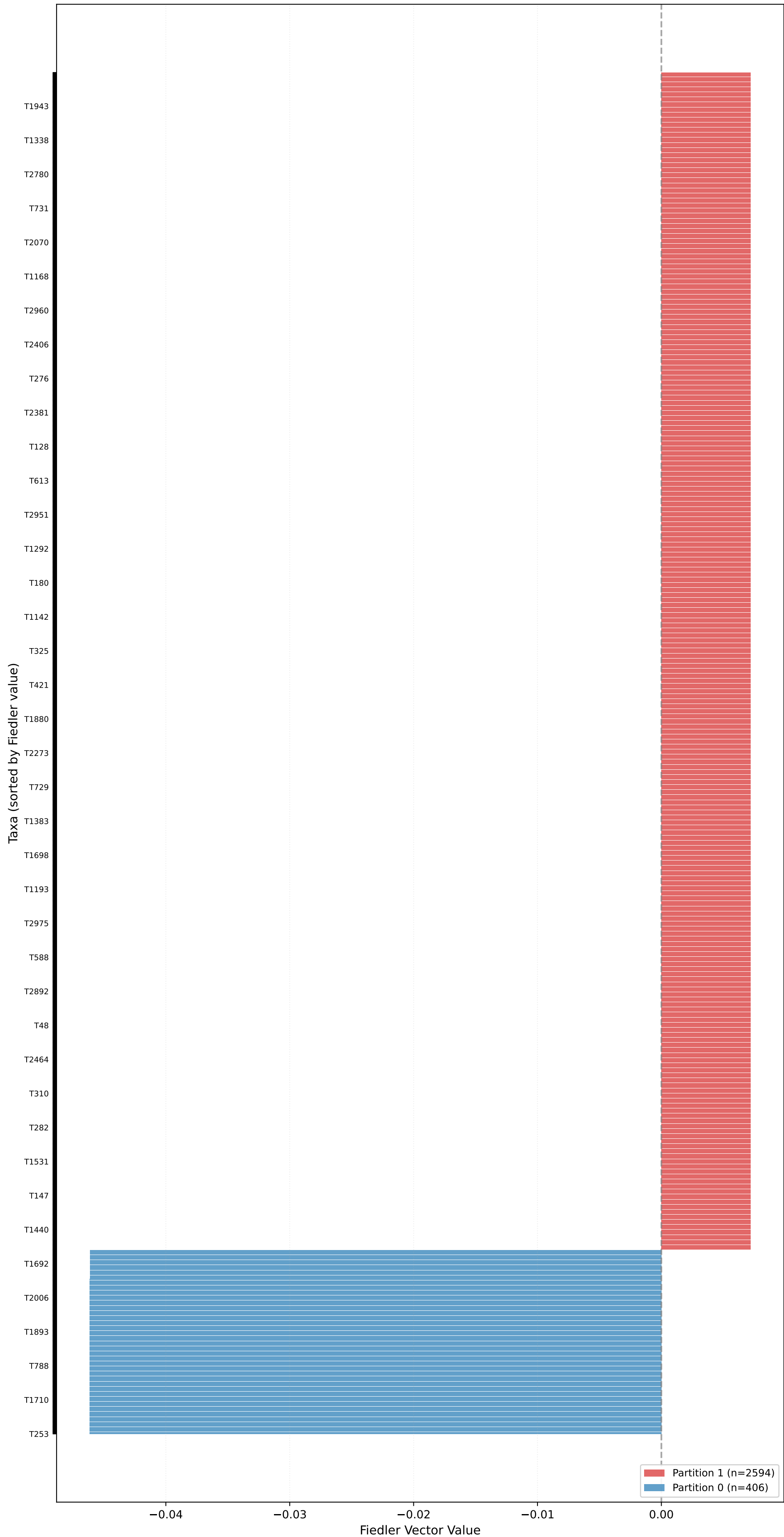
Partition for unrooted_pure_kingman_tree_pop_size_10 (n=3000, L=10000, \mu=0.10 ) - Fiedler Vector \sigma_2=0.0005 , Gap=13.2301, Coherence=0.0025
