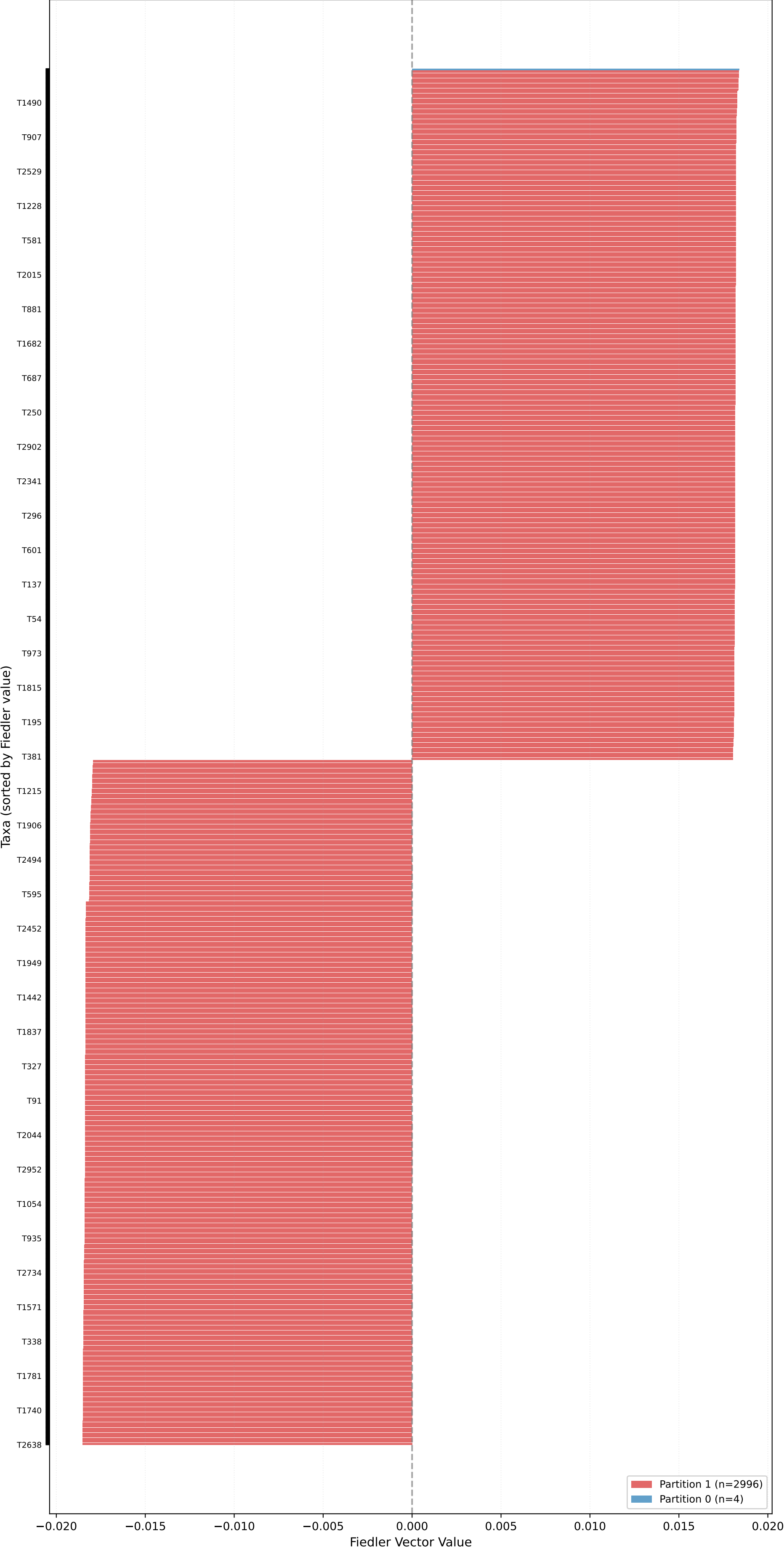
Partition for kingman_mean_pop_1 (n=3000, L=10000, \mu=0.20 ) - Fiedler Vector \sigma_2=0.0070 , Gap=248.2795, Coherence=0.0008
