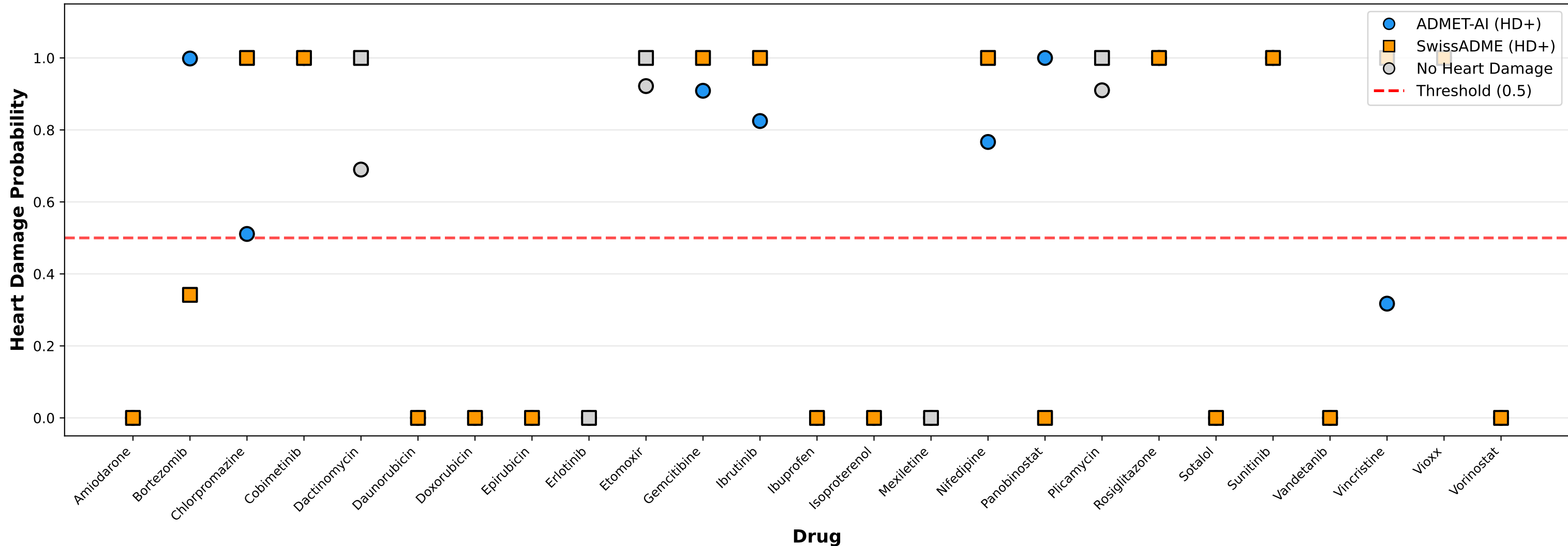
Scaffold-Balanced CV Predictions (25 Drugs)
