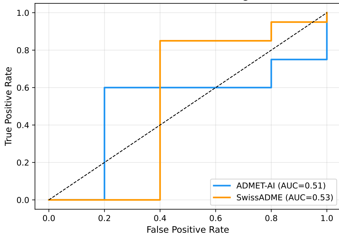
LOOCV Models (25 Cardiac RODEO drugs)
