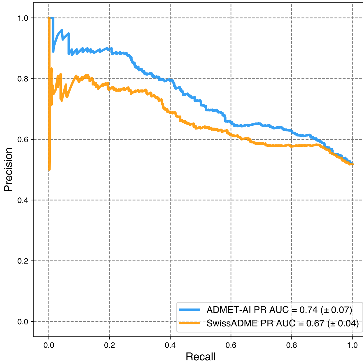
Performance on DICTrank: PR curve
