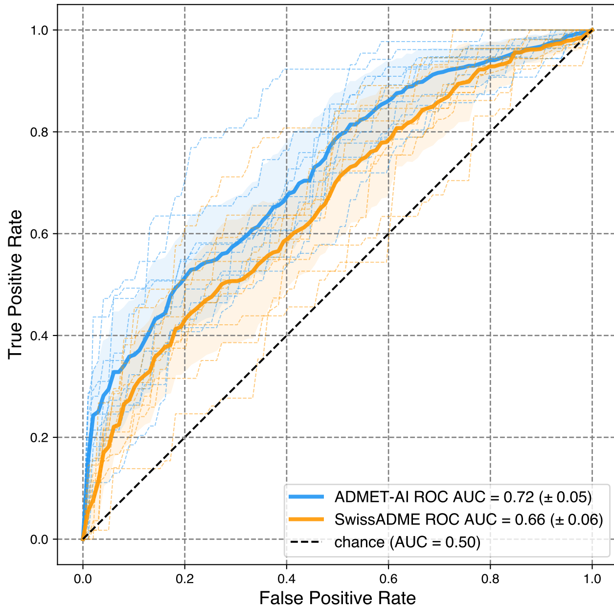
Performance on DICTrank: ROC curve
