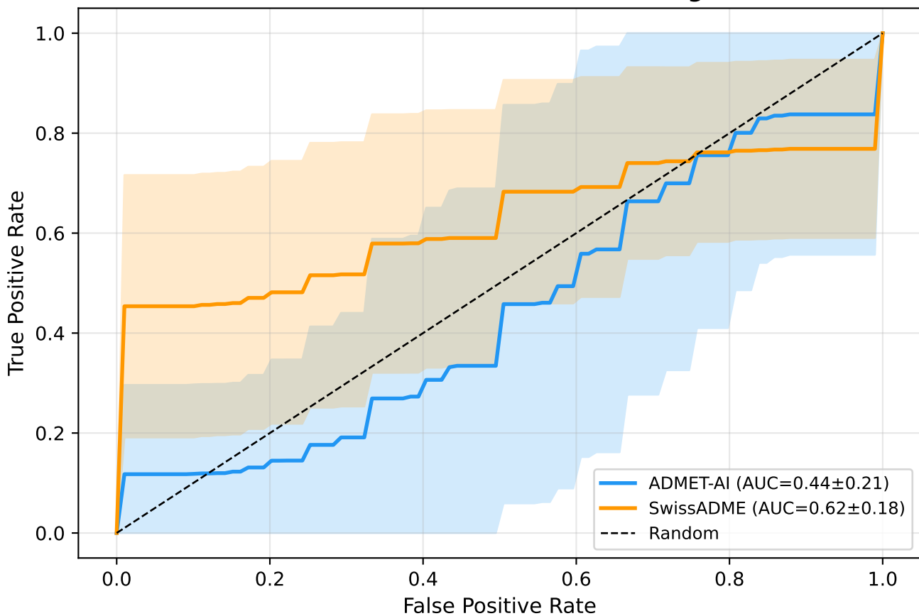
DICTrank ROC Curves on 25 Drugs
