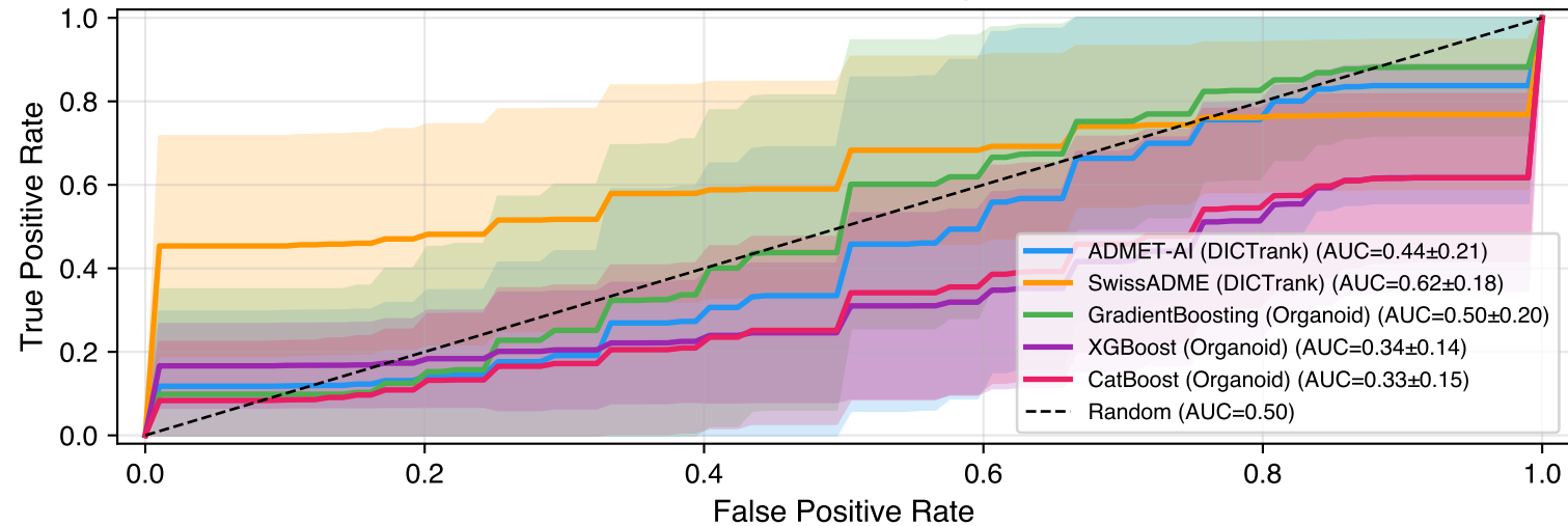
ROC Curves: DICTrank vs Organoid Models
