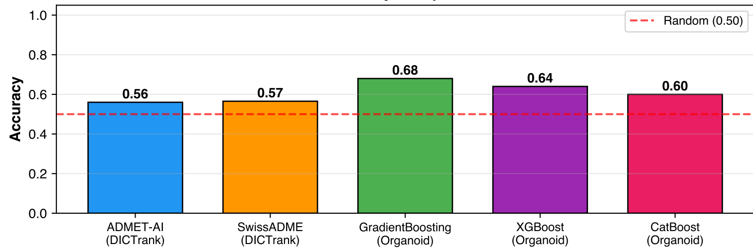
Accuracy Comparison
