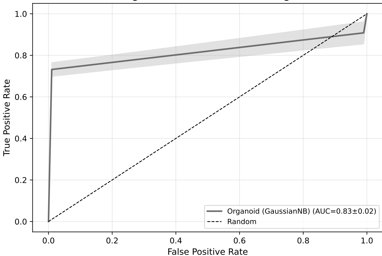
Organoid ROC Curve on 25 Drugs
