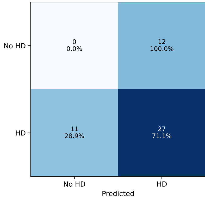
ADMET-AI Accuracy: 0.54
