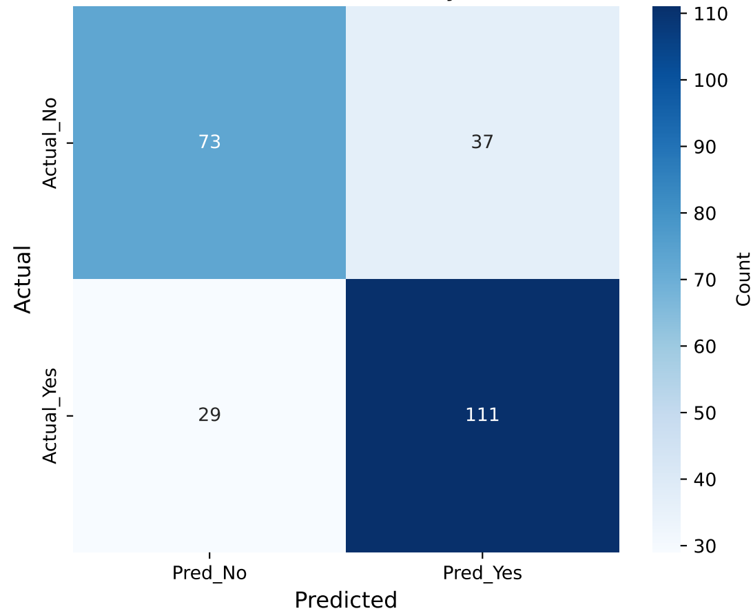
Confusion Matrix: Arrhythmia
