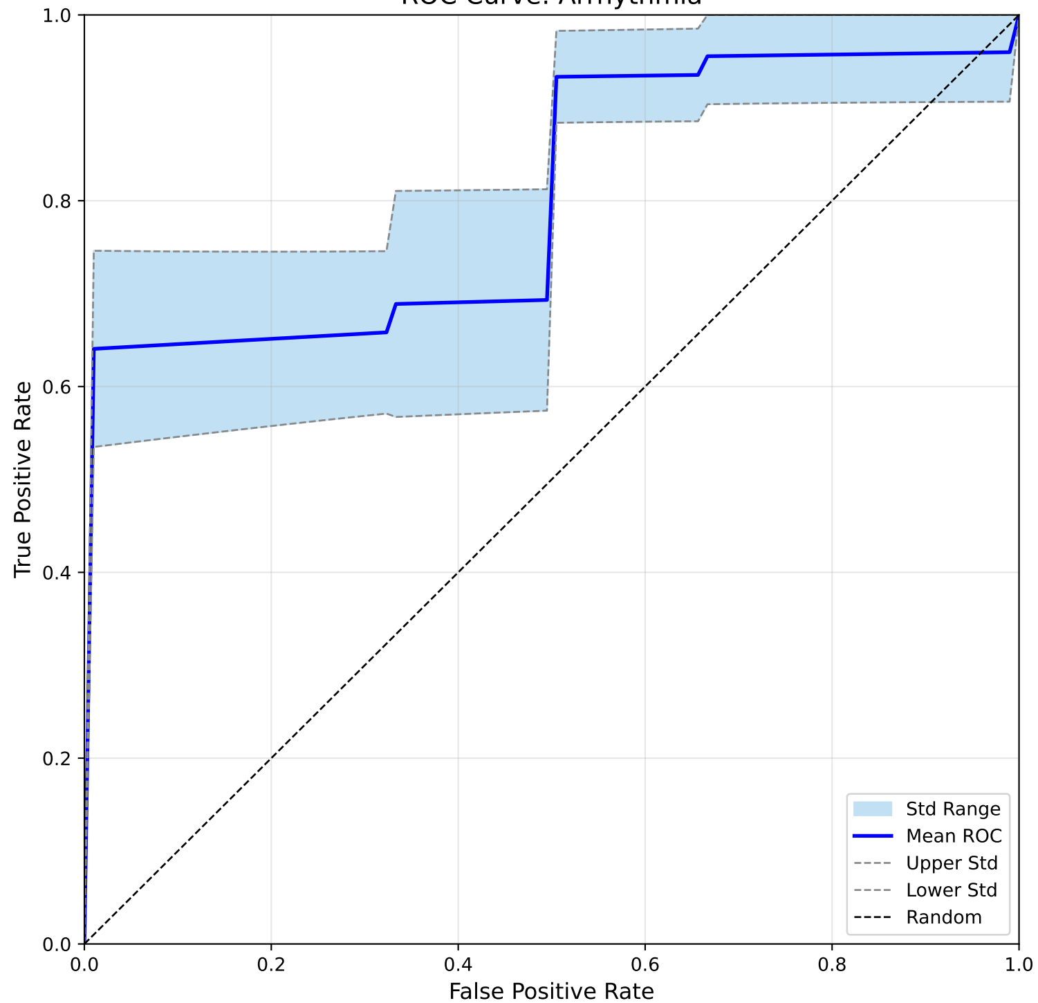
ROC Curve: Arrhythmia
