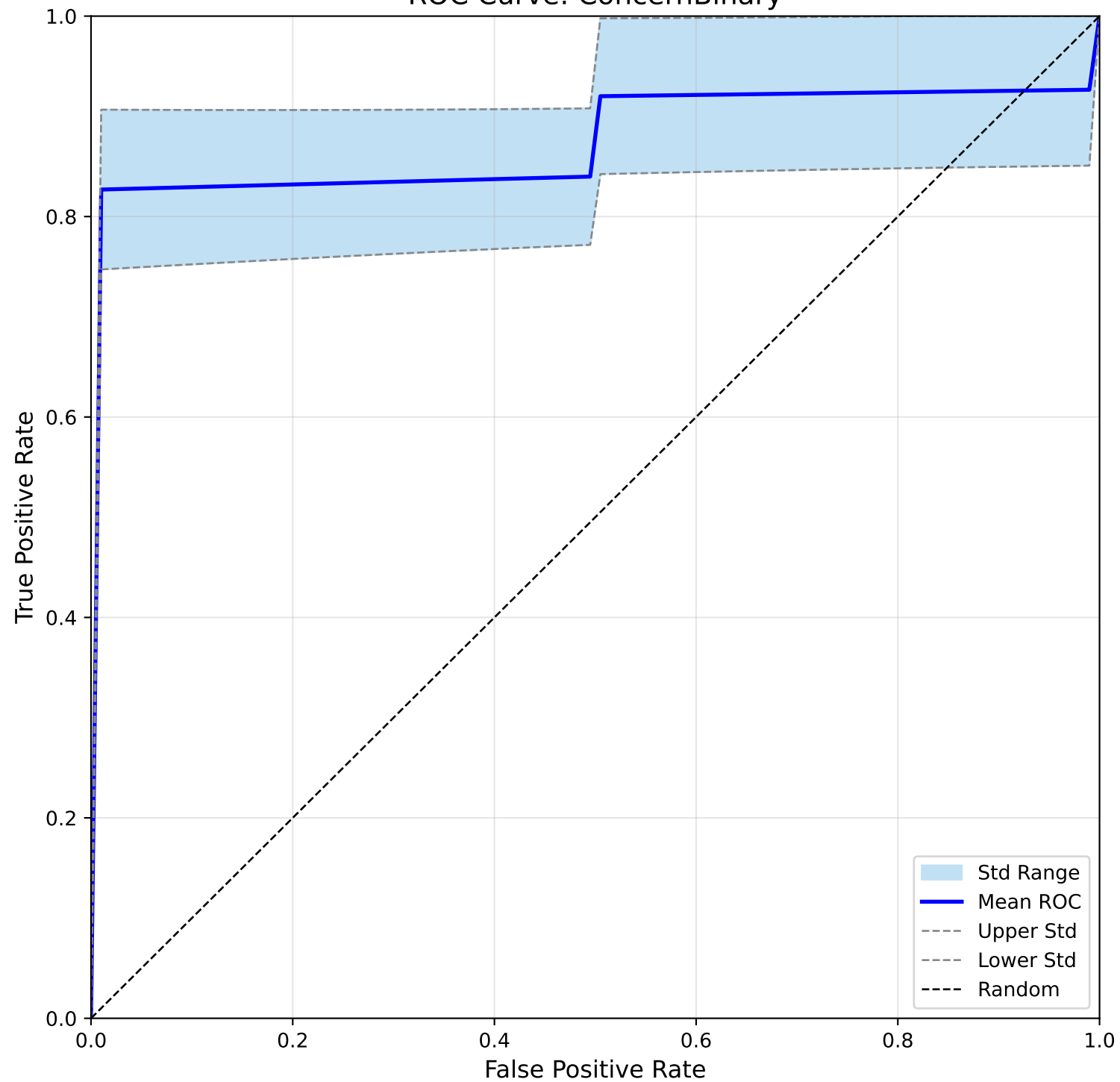
ROC Curve: ConcernBinary
