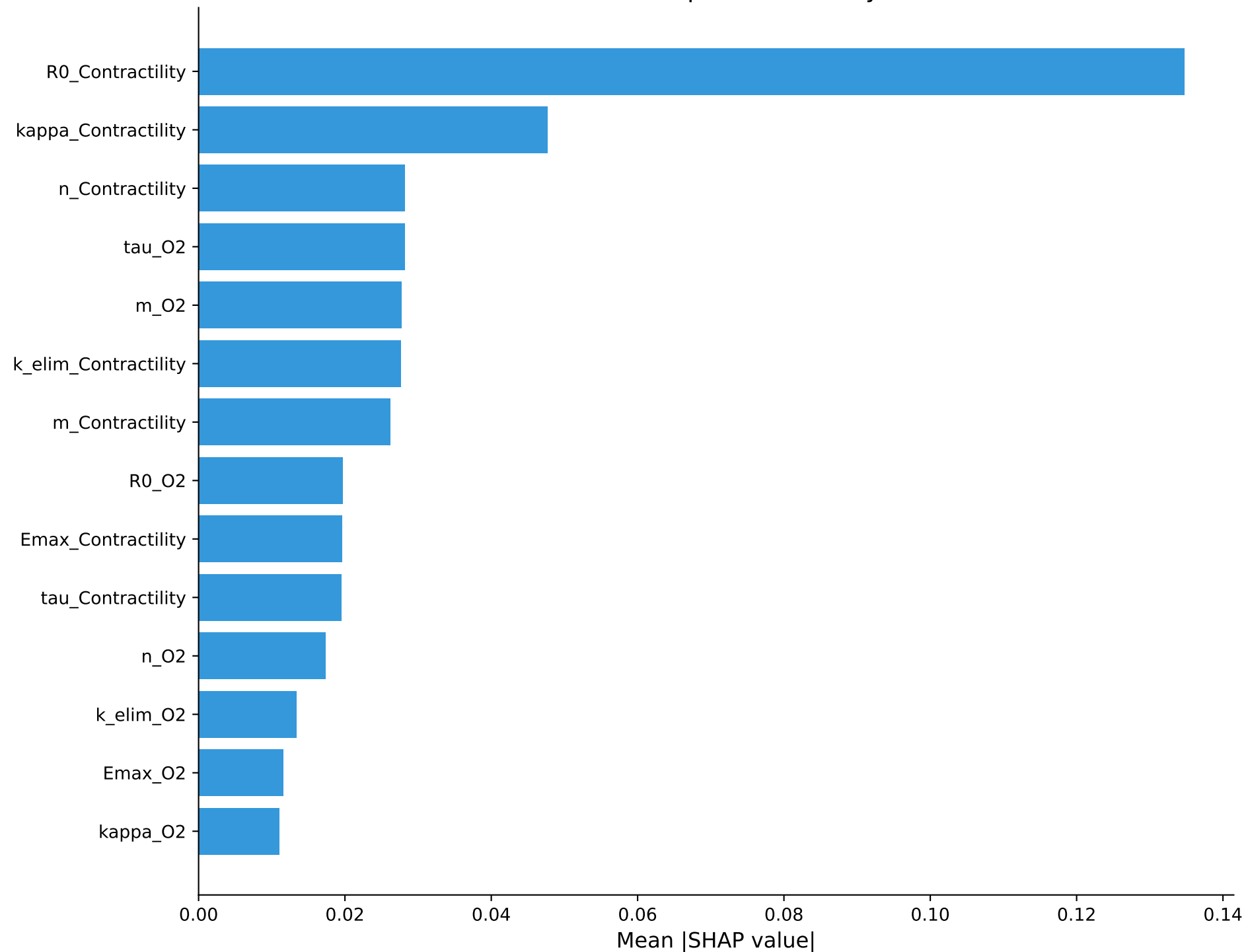
SHAP Feature Importance: Arrhythmia
