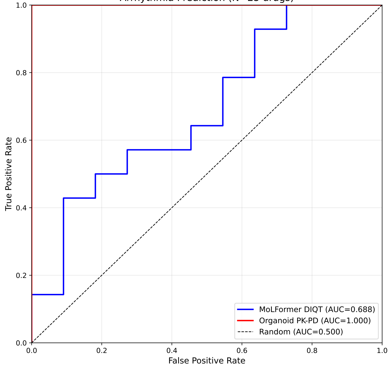
ROC Comparison: MoLFormer vs Organoid Arrhythmia Prediction (N=25 drugs)
