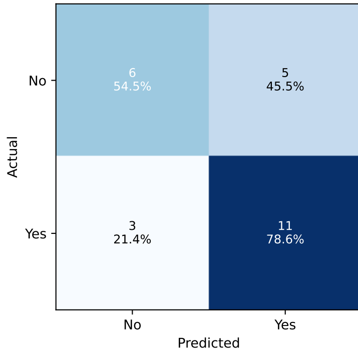
CNN (5-fold on 25) (Acc=0.68)
