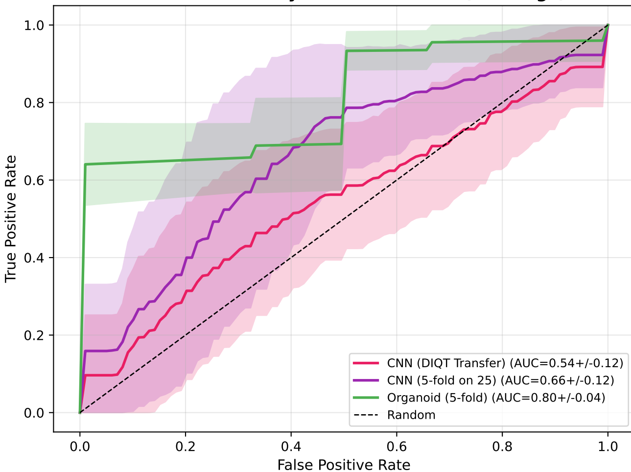
ROC Curves: Arrhythmia Prediction (25 Drugs)
