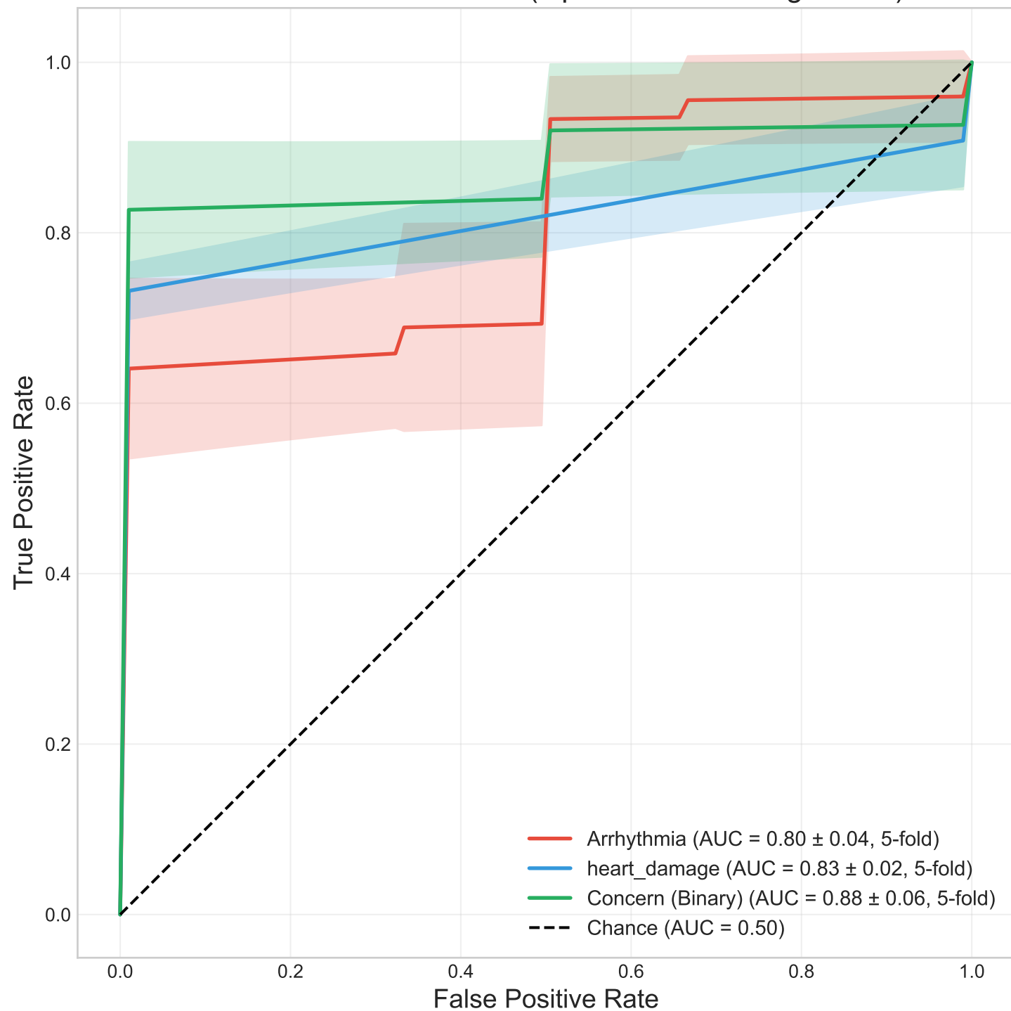
Final Model ROC Curves (Optimal Fold Configuration)
