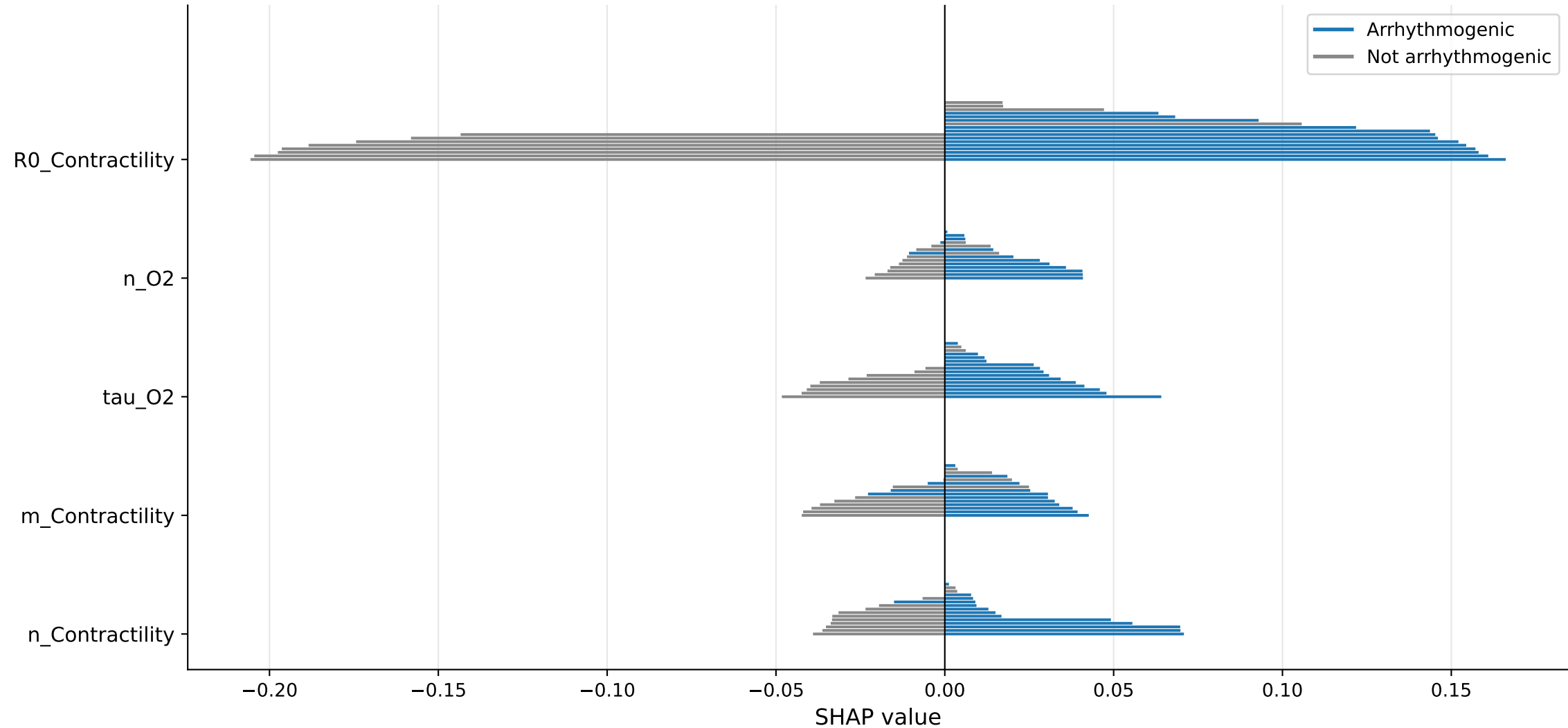
Aligned positive-negative SHAP pairs per feature
