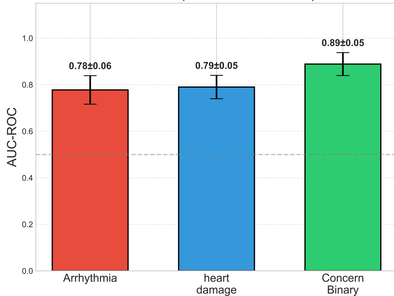
AUC-ROC (10 Seeds × 4-Fold CV)
