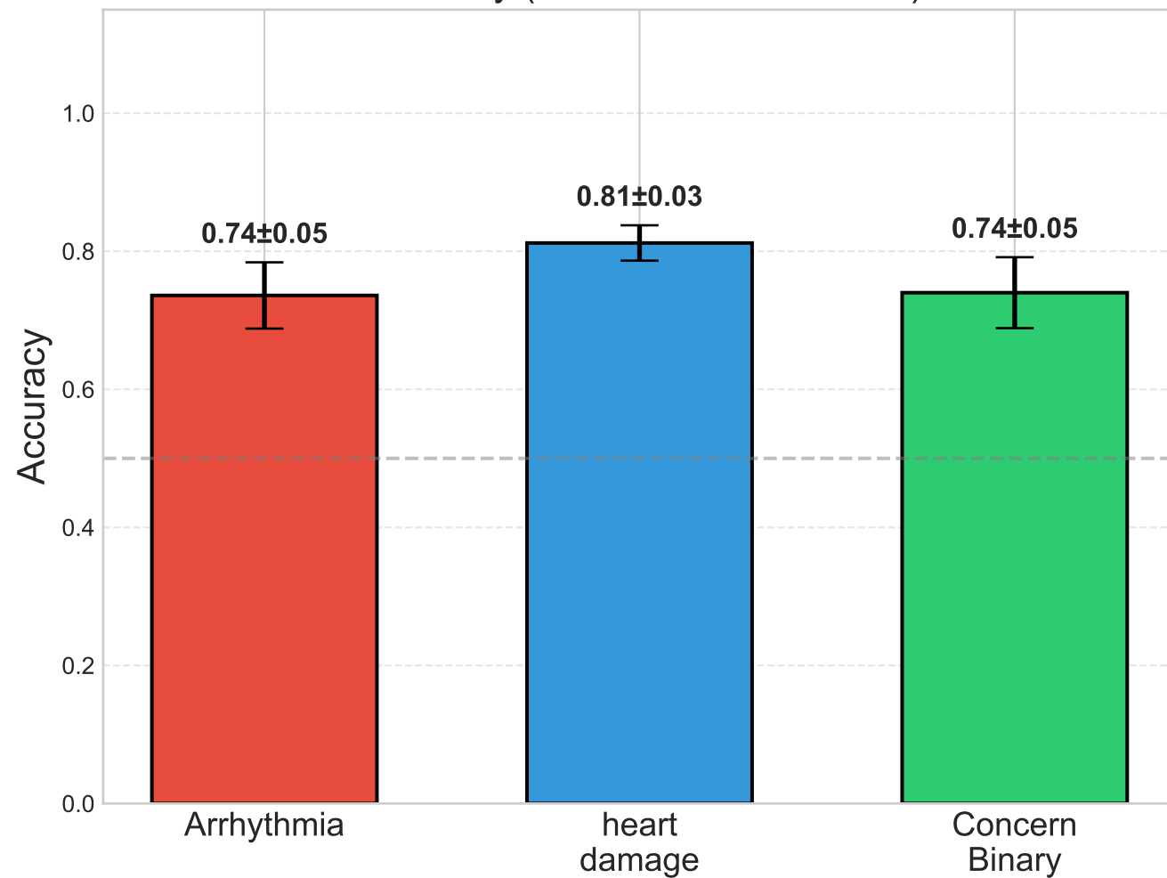
Accuracy (10 Seeds × 5-Fold CV)
