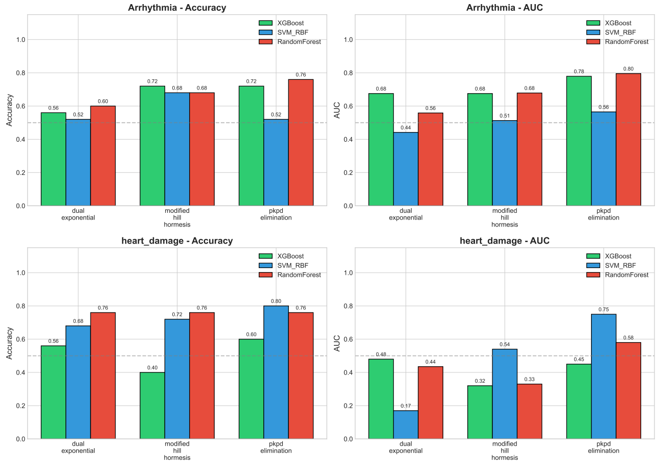
Figure 1: Stage 1 LOOCV performance for Arrhythmia and Heart Damage prediction.
