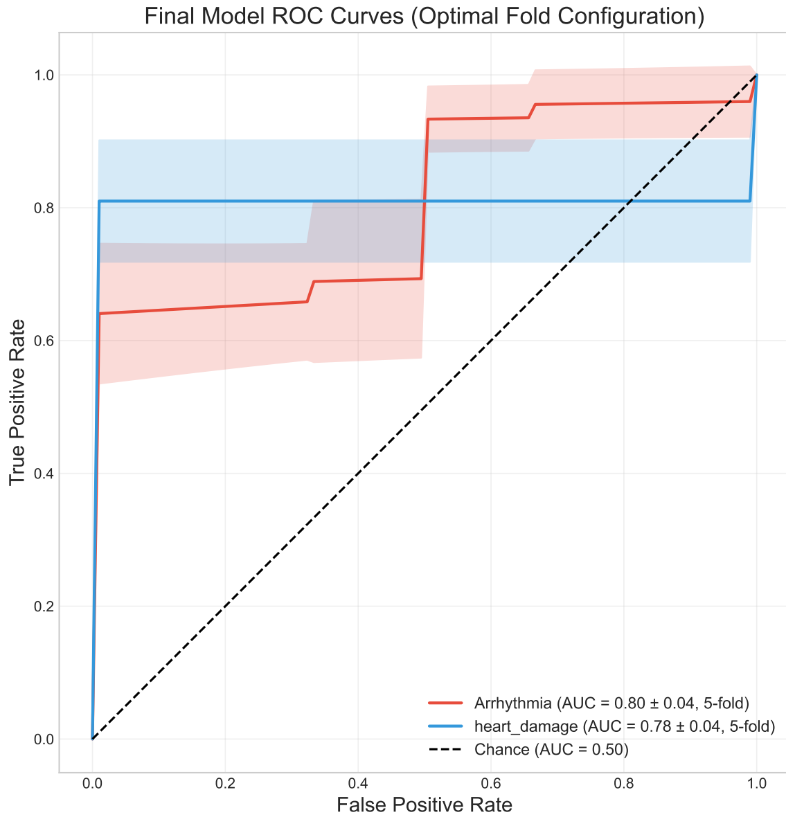
Figure 12: ROC curves for final model configurations with optimal fold counts.
