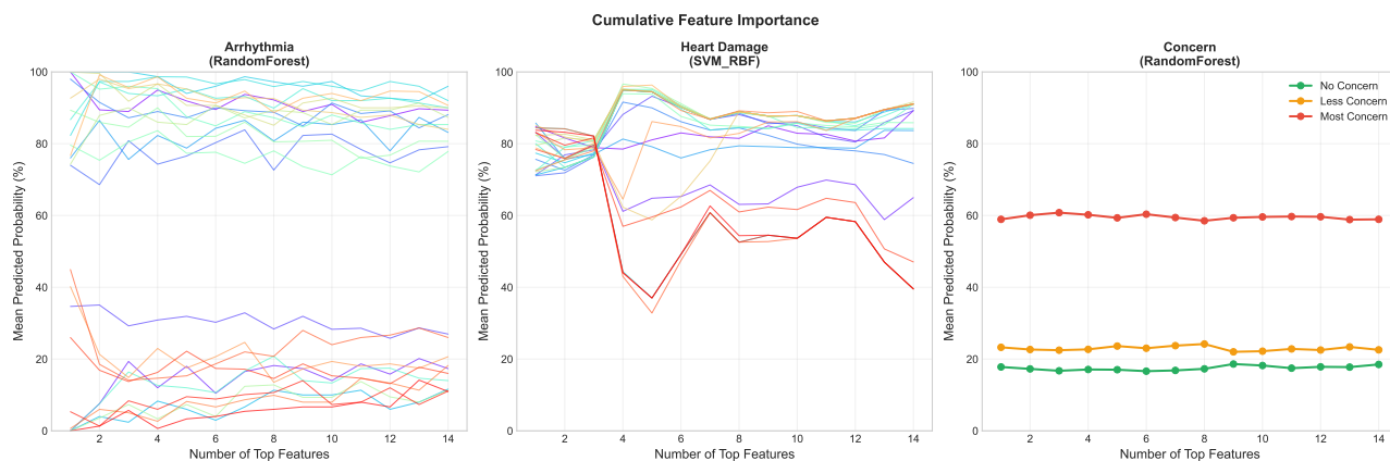
Figure 15: Cumulative feature importance showing how prediction probability changes as features are added.
