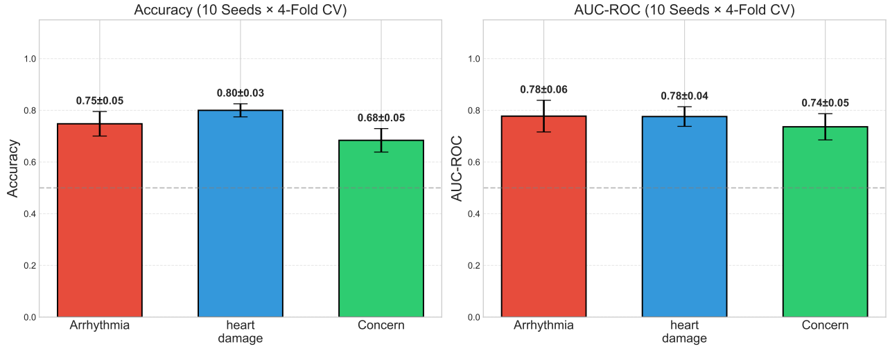
Figure 7: Accuracy and AUC for 4-Fold CV with error bars ( \pm 1 std).
