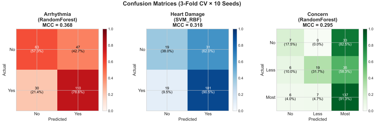
Figure 5: Confusion matrices for 3-Fold CV (aggregated across 10 seeds).
