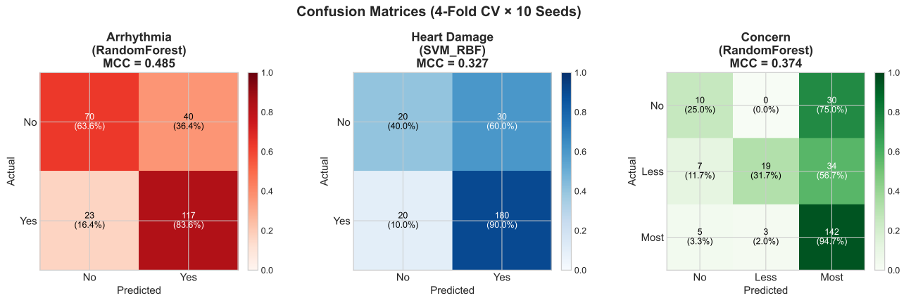
Figure 8: Confusion matrices for 4-Fold CV (aggregated across 10 seeds).
