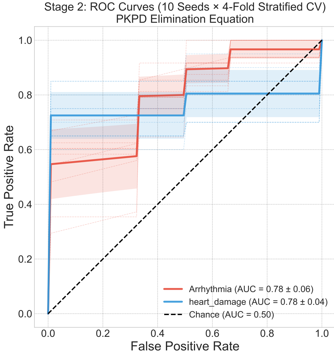
Figure 6: ROC curves for 4-Fold CV showing mean \pm std bands across 10 seeds.
