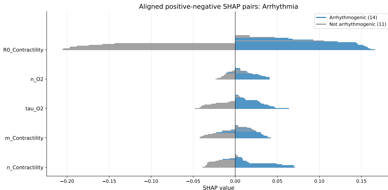
Figure 16: Aligned SHAP pairs for Arrhythmia prediction. Blue lines = arrhythmogenic drugs (14), grey lines = non-arrhythmogenic drugs (11). The alignment of blue lines on the right (positive SHAP) and grey on the left (negative SHAP) indicates good model discrimination. All 25 drugs shown for each feature (no exclusions).
