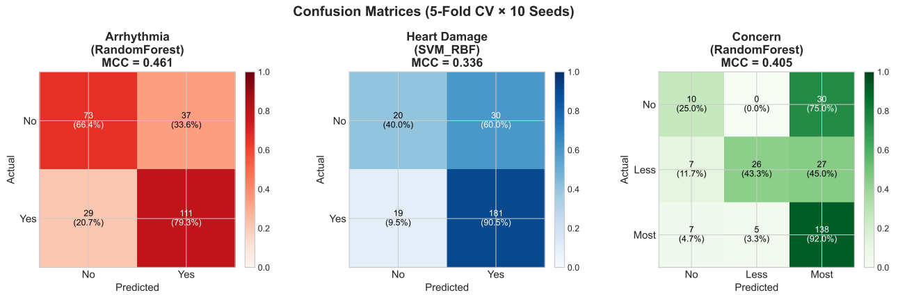
Figure 11: Confusion matrices for 5-Fold CV (aggregated across 10 seeds).
