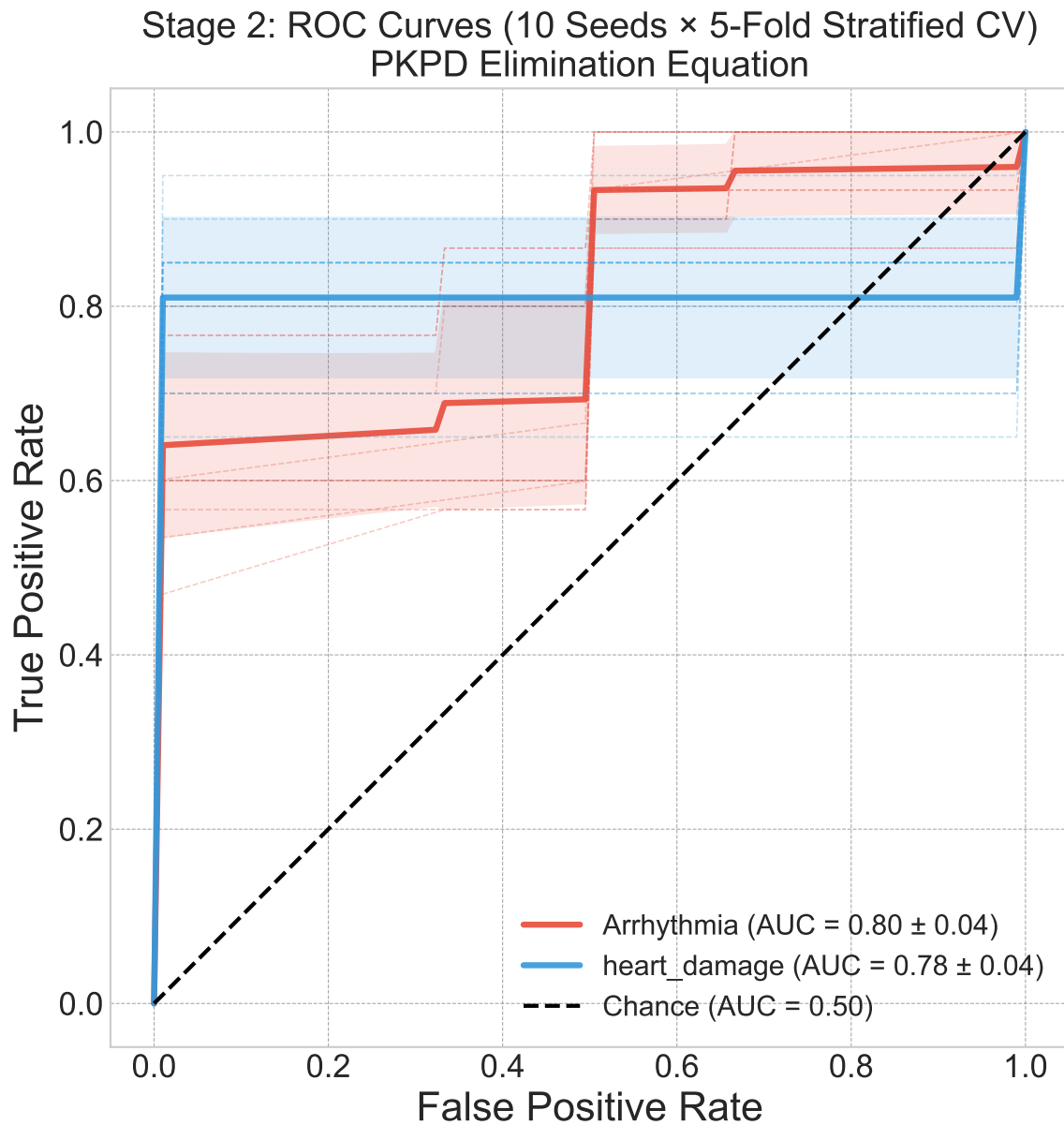
Figure 9: ROC curves for 5-Fold CV showing mean \pm std bands across 10 seeds.
