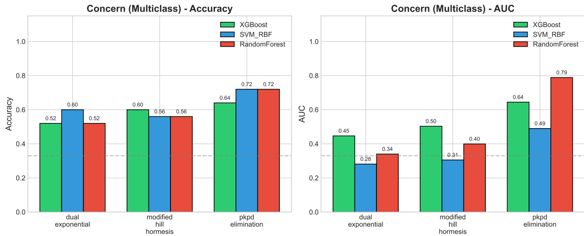
Figure 2: Stage 1 LOOCV performance for Concern level prediction (multiclass).
