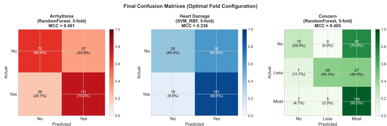
Figure 13: Confusion matrices for final model configurations.
