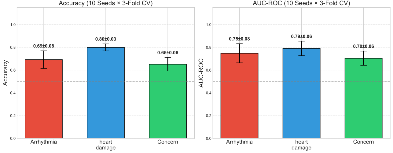
Figure 4: Accuracy and AUC for 3-Fold CV with error bars ( \pm 1 std).
