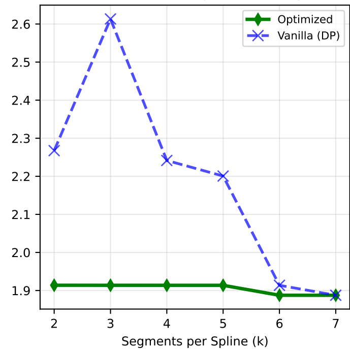
Medium-2 -- functionexp100 (1,010 params)
