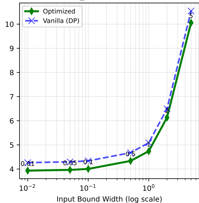
Large -- acopf_ml4acopf (53,248 params)
