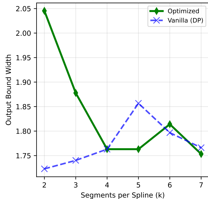
Small -- pinnheat (420 params)
