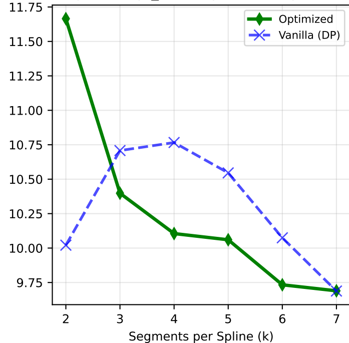
Large -- acopf_ml4acopf (53,248 params)
