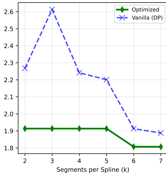
Medium -- functionexp100 (1,010 params)
