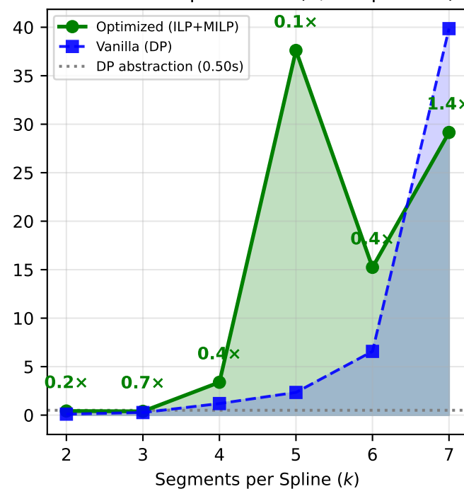
Medium-2 -- prosthetic (3,616 params)
