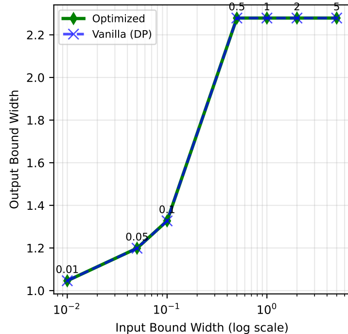
Small -- functionbessel (20 params)
