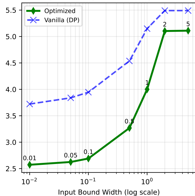
Large -- funcsppharm (140 params)
