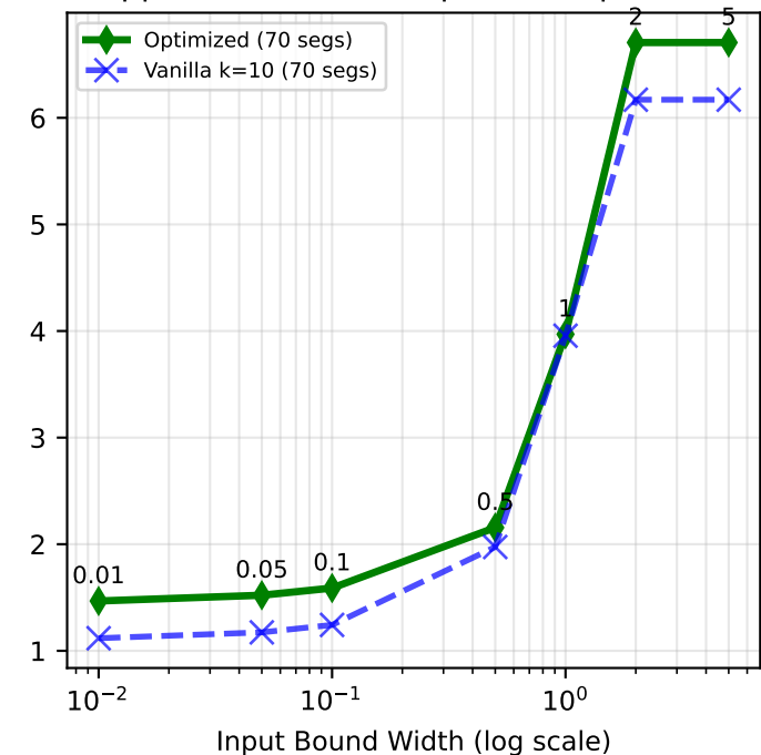
Appendix-3 -- funcellipkinc (70 params)
