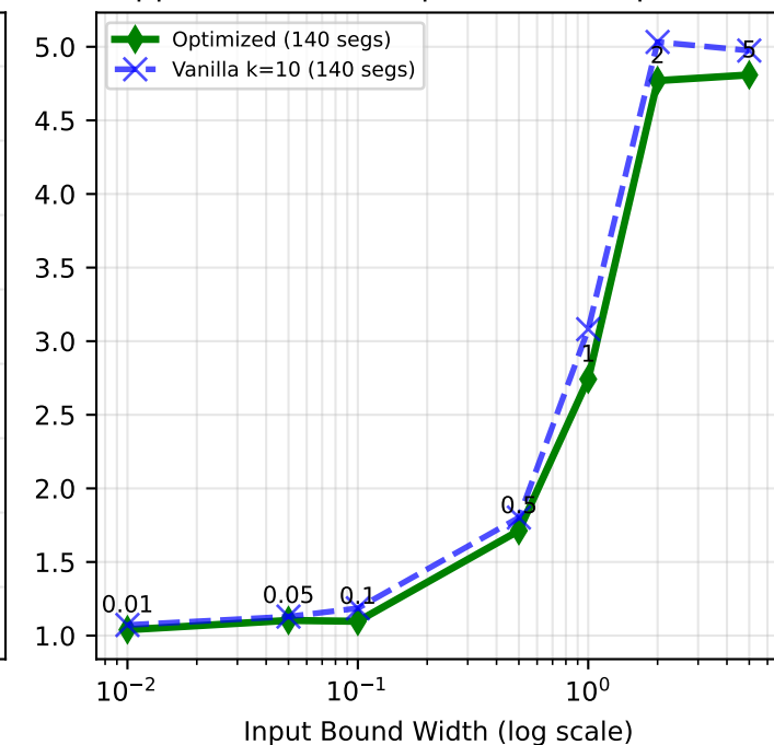
Appendix-5 -- funcsphharm (140 params)
