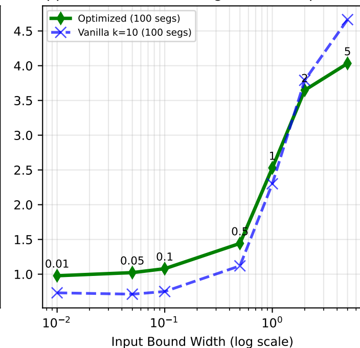
Appendix-4 -- functionlegendre (100 params)
