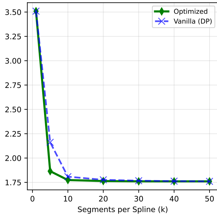
Large -- functionexp100 (1,010 params)
