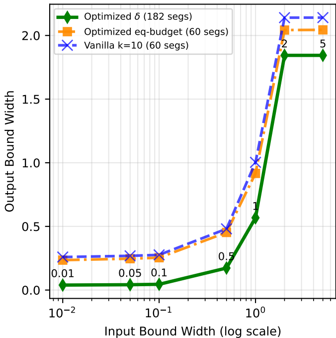
Small -- functionxy (60 params)
