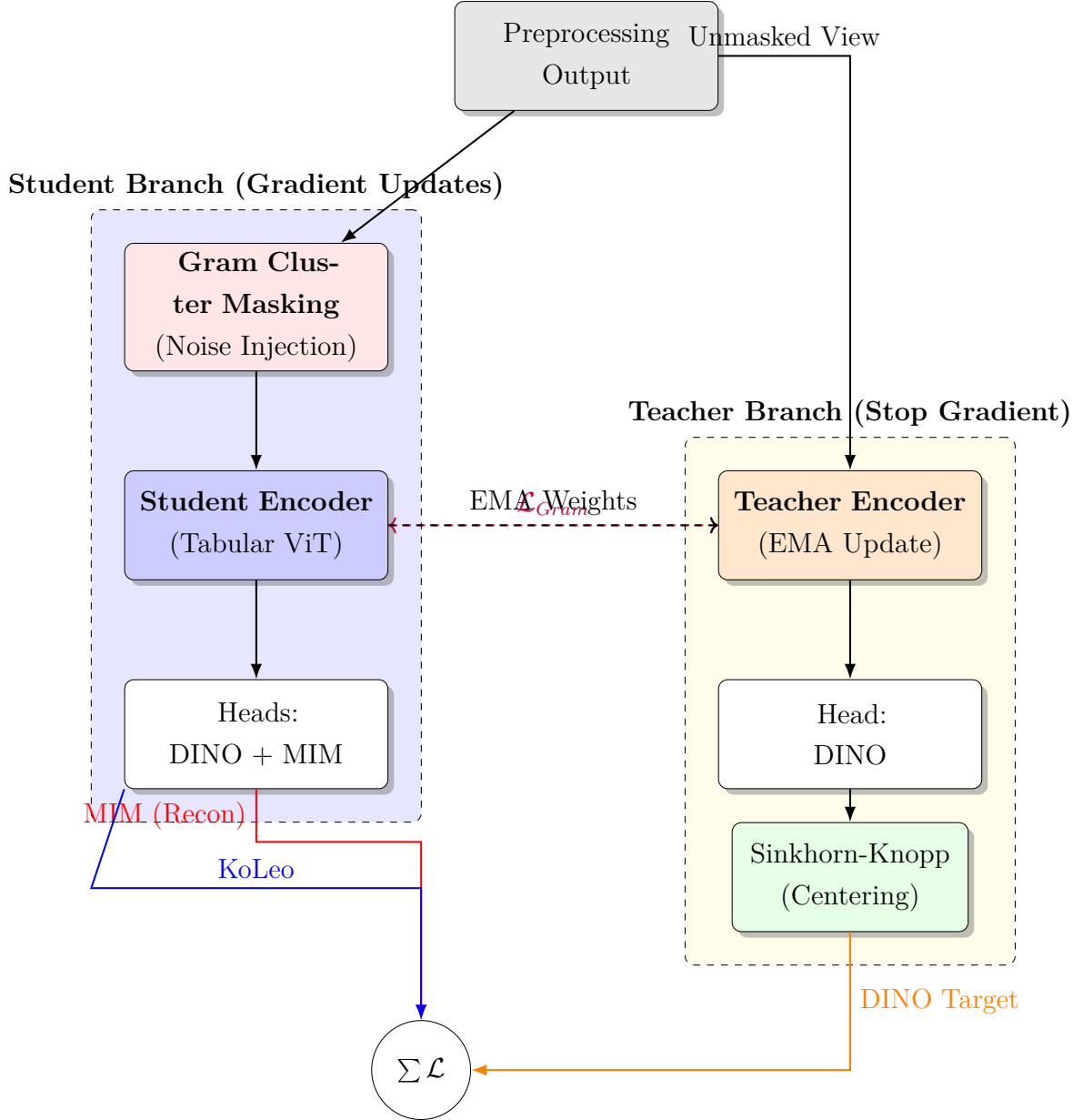
Figure 2.2: The DINOv3 Architecture adapted for Tabular Data. The Student learns from a corrupted view, guided by the stable Teacher. The Sinkhorn-Knopp algorithm prevents mode collapse, while the Gram Loss ensures structural consistency.
