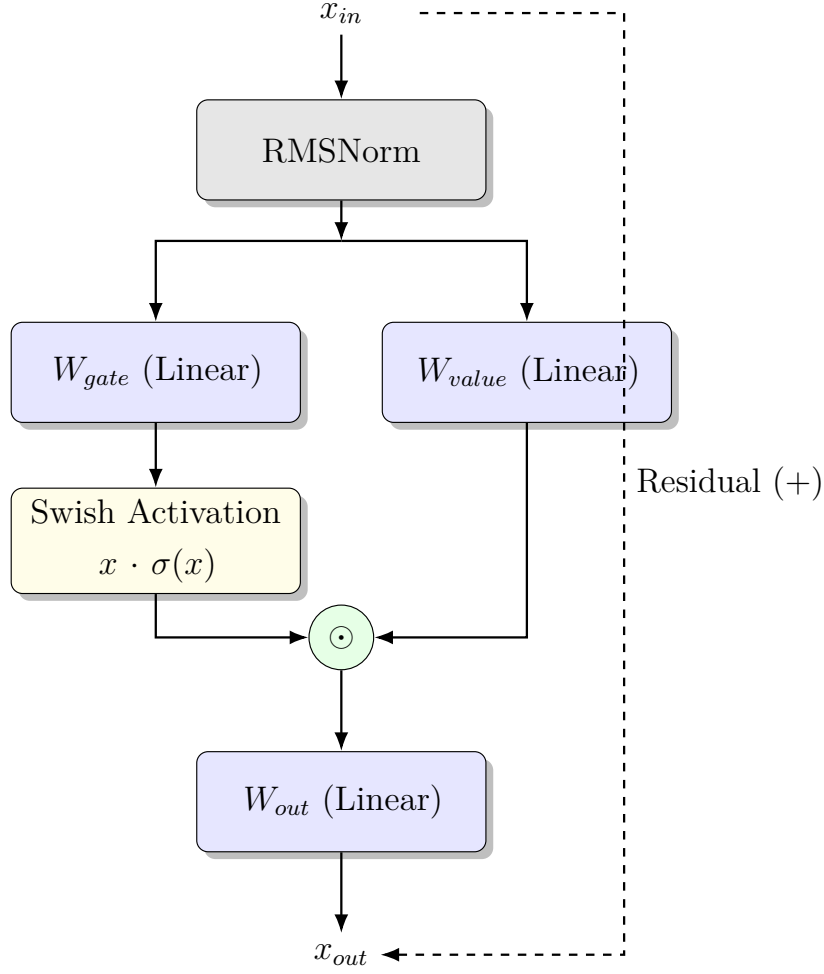
Figure 2.3: The SwiGLU Block structure. The gating mechanism allows the network to control information flow, enabling deeper architectures to converge faster.
