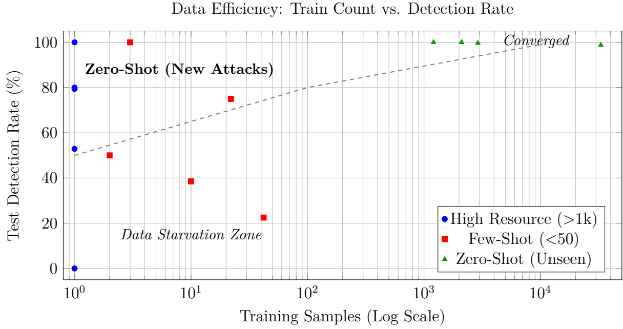
Figure 4.1: The Generalization Frontier. Points at x \approx 10^0 represent Zero-Shot attacks (0 training samples). The high variance in this zone indicates that while the model generalizes well to some unknown signatures (SqlAttack), it fails on others (Mailbomb), highlighting the need for future Few-Shot Learning augmentation.
