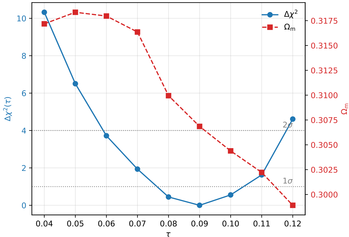
CMB 2pt: Planck PR4 ( 30 < \ell < 1000 ) + ACT DR6 ( \ell > 1000 ) + SPT-3G D1
