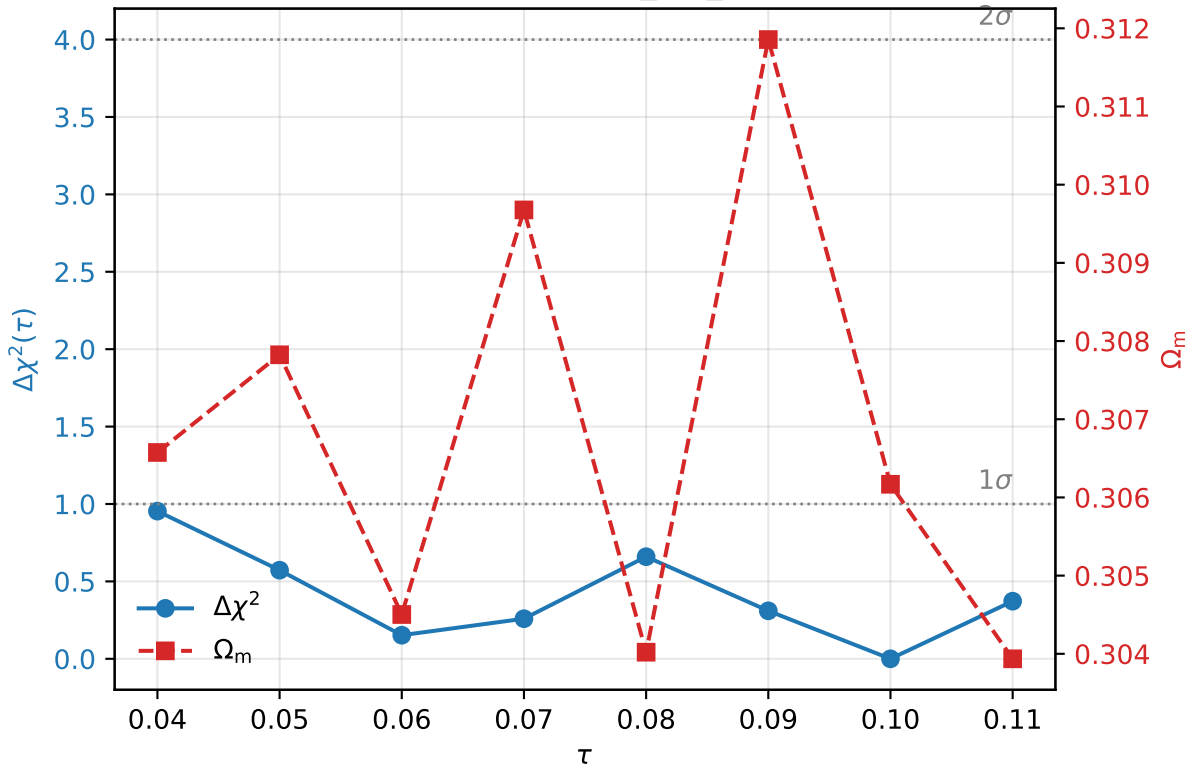
CMB 2pt: cmb2pt_lite_alens
