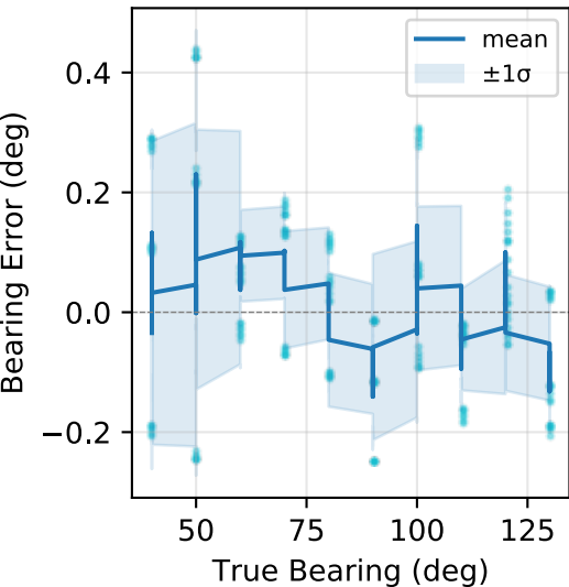
Bearing error vs true bearing
