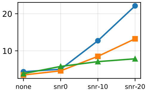
MOTP (m)
