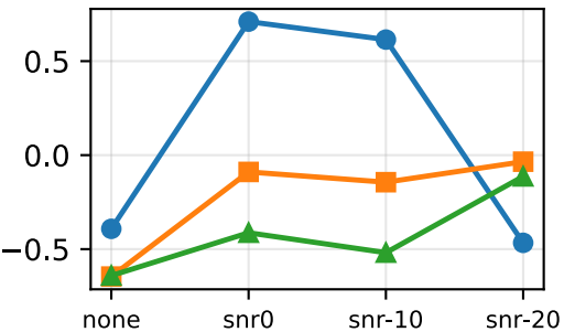
MOTA
