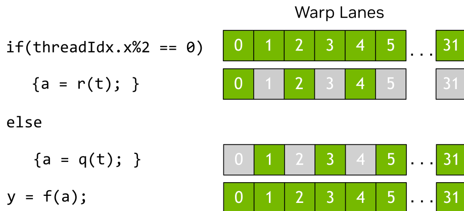
FIGURE 2.8: In this example, branching paths in execution between the even and odd threads prevent all threads from executing in parallel. All even threads execute the top branch while all odd threads are idle, then vice versa. As a result, the execution time is the sum of the two branches instead of the maximum. Source: [26].
