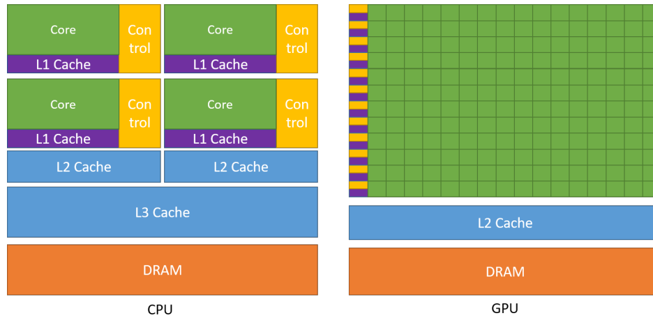
FIGURE 2.7: The GPU devotes more transistors to data processing than the CPU. Each (green) core acts as a thread that executes the same instruction on different data elements. Source: [26].
